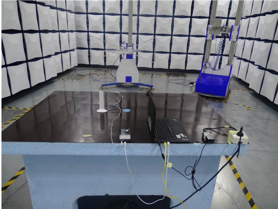
Radiated Disturbance Emissions (below 1GHz)
