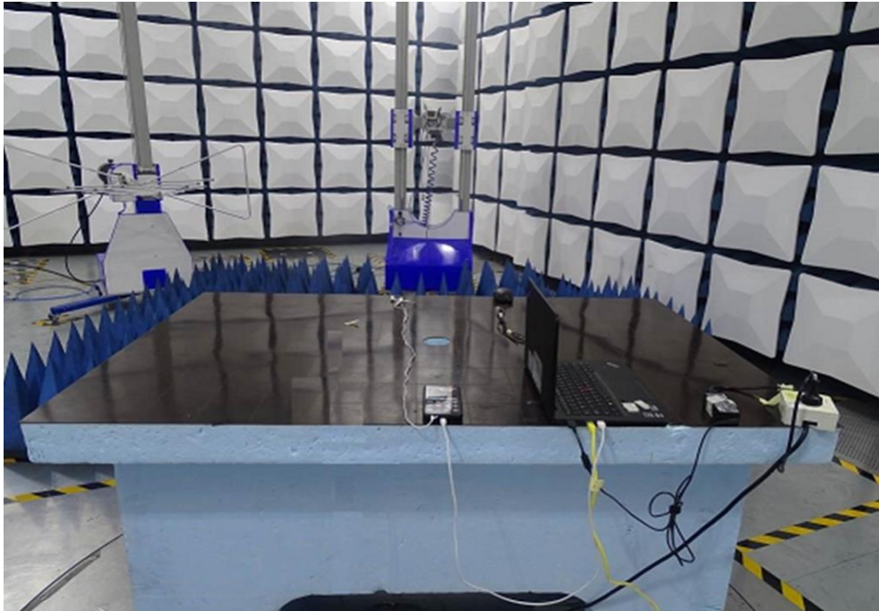
Radiated Disturbance Emissions (18GHz to 26.5GHz)
