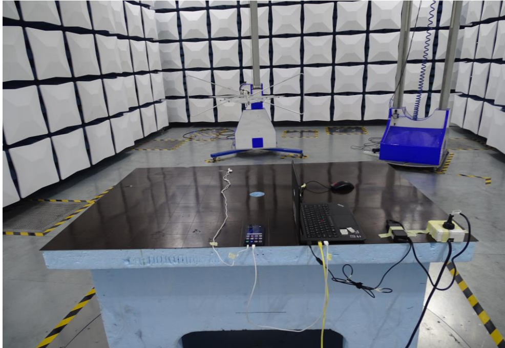
Radiated Disturbance Emissions (below 1GHz)
