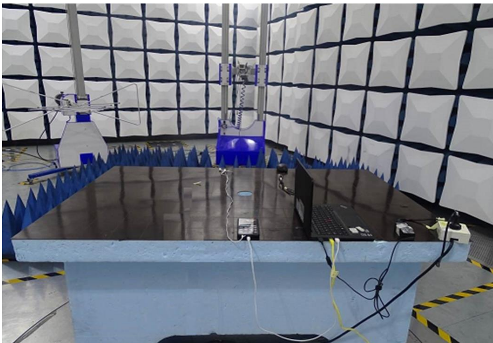
Radiated Disturbance Emissions (26.5GHz to 40GHz)
