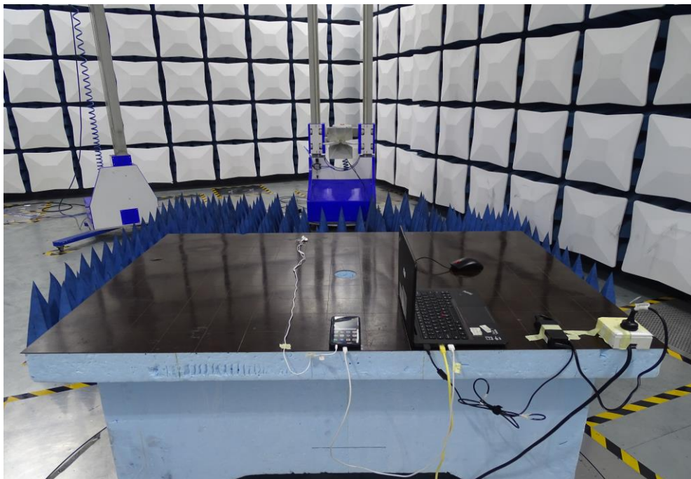
Radiated Disturbance Emissions (1GHz to 18GHz)
