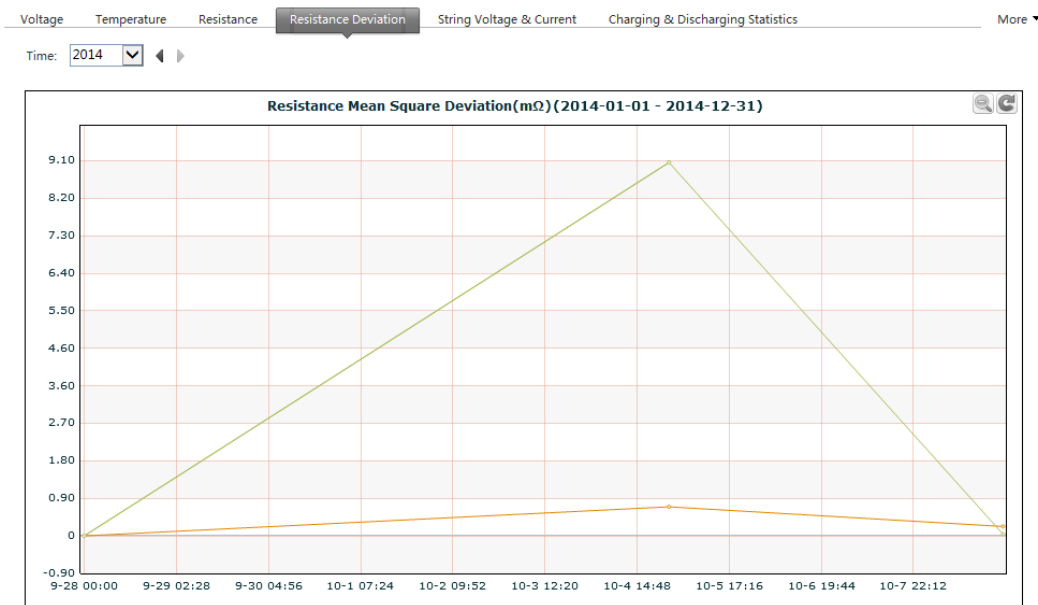
Figure 3-8 Historical battery resistance deviation
