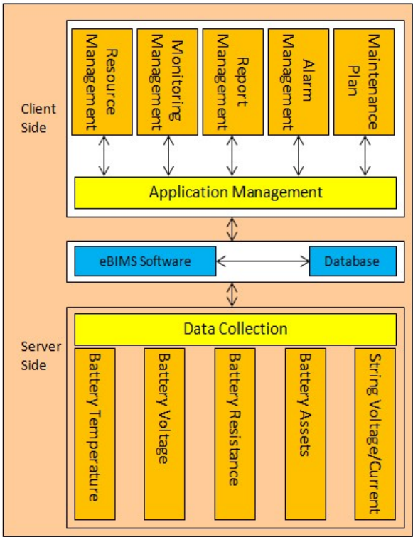
Figure 2-6 Software architecture of the eBIMS
