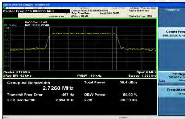
Part 90_Band26_3MHz_16QAM_15_0_HighCH26775
