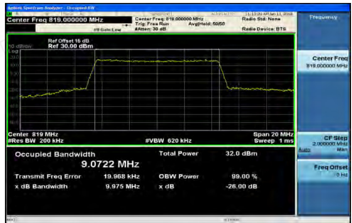
Part 90_Band26_10MHz_16QAM_50_0_MidCH26740
