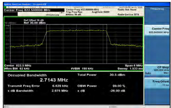
Part 90_Band26_3MHz_64QAM_15_0_HighCH26775
