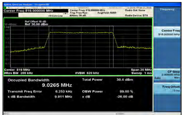
Part 90_Band26_10MHz_64QAM_50_0_MidCH26740
