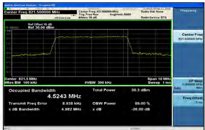
Part 90_Band26_5MHz_16QAM_25_0_HighCH26765
