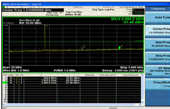
30MHz~3GHz_Band26_5MHz_QPSK_1_0_HighCH26765
