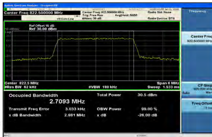
Part 90_Band26_3MHz_QPSK_15_0_HighCH26775
