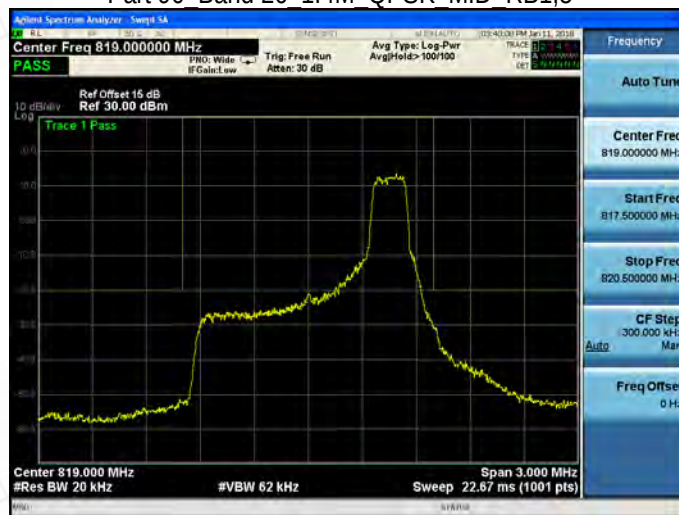
Part 90 Band 26 1.4M QPSK MID RB6,0
