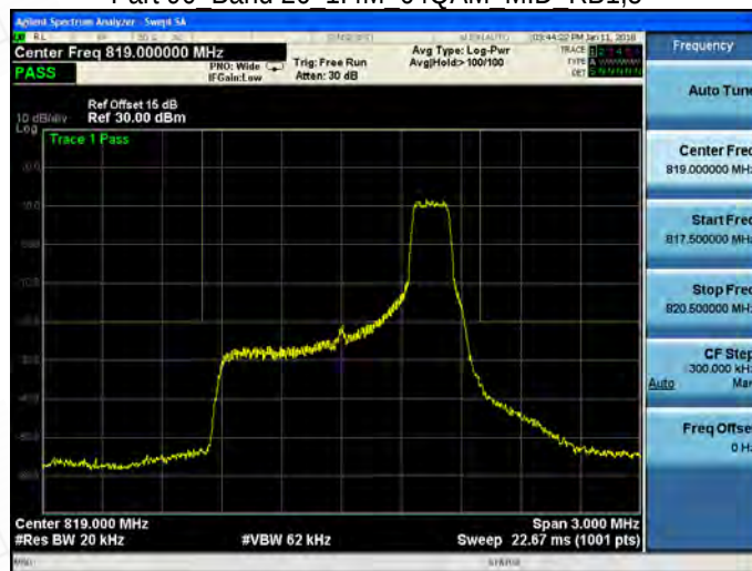
Part 90 Band 26 1.4M 64QAM MID RB6,0
