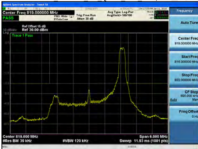
Part 90 Band 26 3M QPSK MID RB15,0
