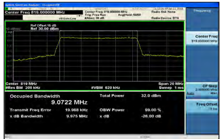
Part 90_Band26_10MHz_16QAM_50_0_MidCH26740
