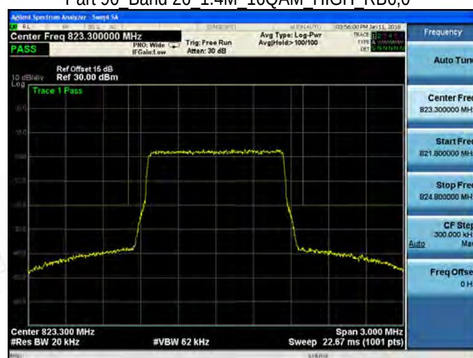
Part 90 Band 26 1.4M 16QAM HIGH RB6,0
