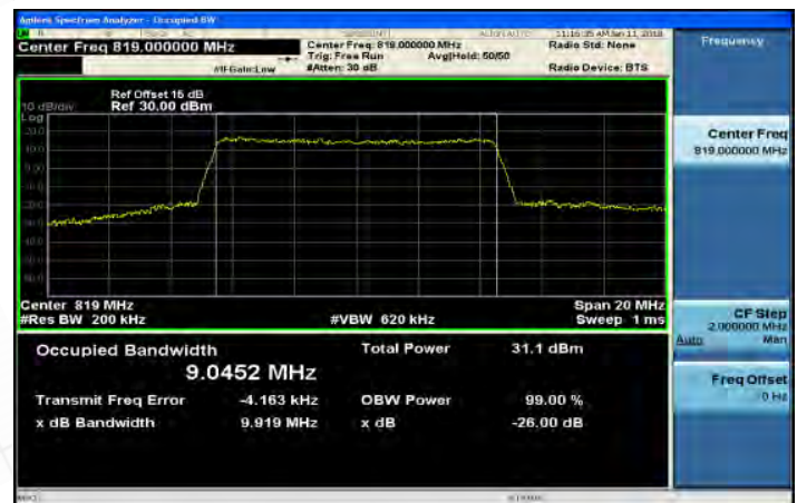
Part 90_Band26_10MHz_64QAM_50_0_MidCH26740
