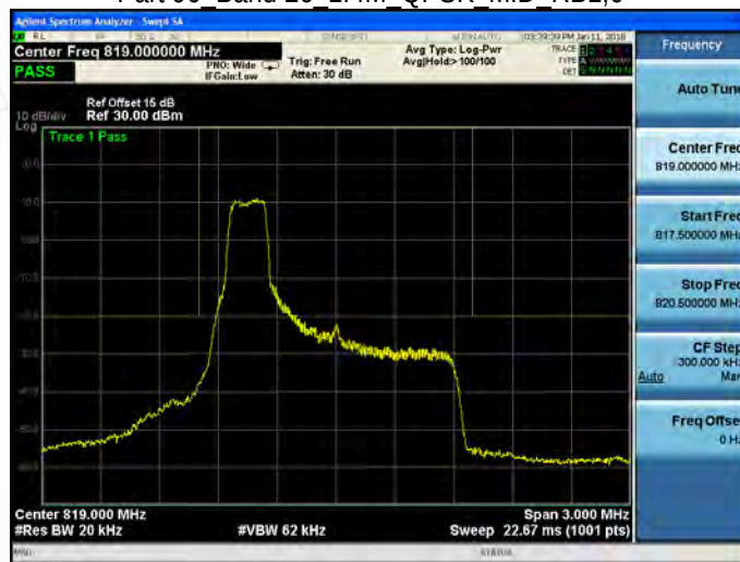
Part 90 Band 26 1.4M QPSK MID RB1,5
