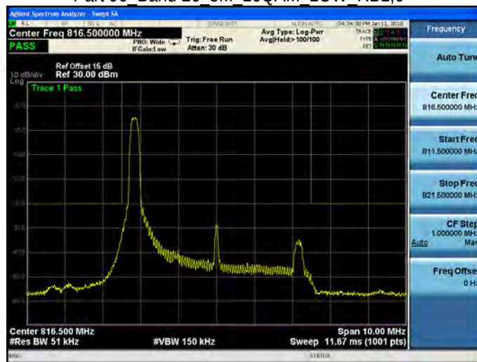
Part 90 Band 26 5M 16QAM LOW RB1,24
