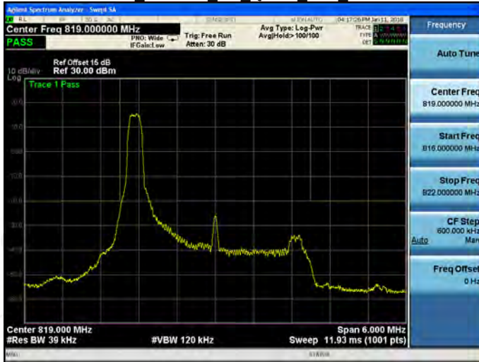
Part 90 Band 26 3M QPSK MID RB1,14
