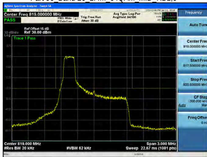
Part 90 Band 26 1.4M 64QAM MID RB1,5
