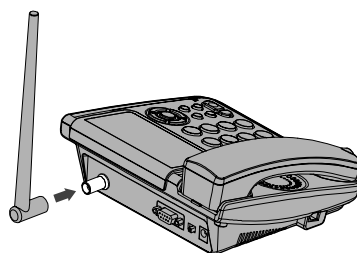
Figure 1 installing an antenna for the fixed wireless terminal
