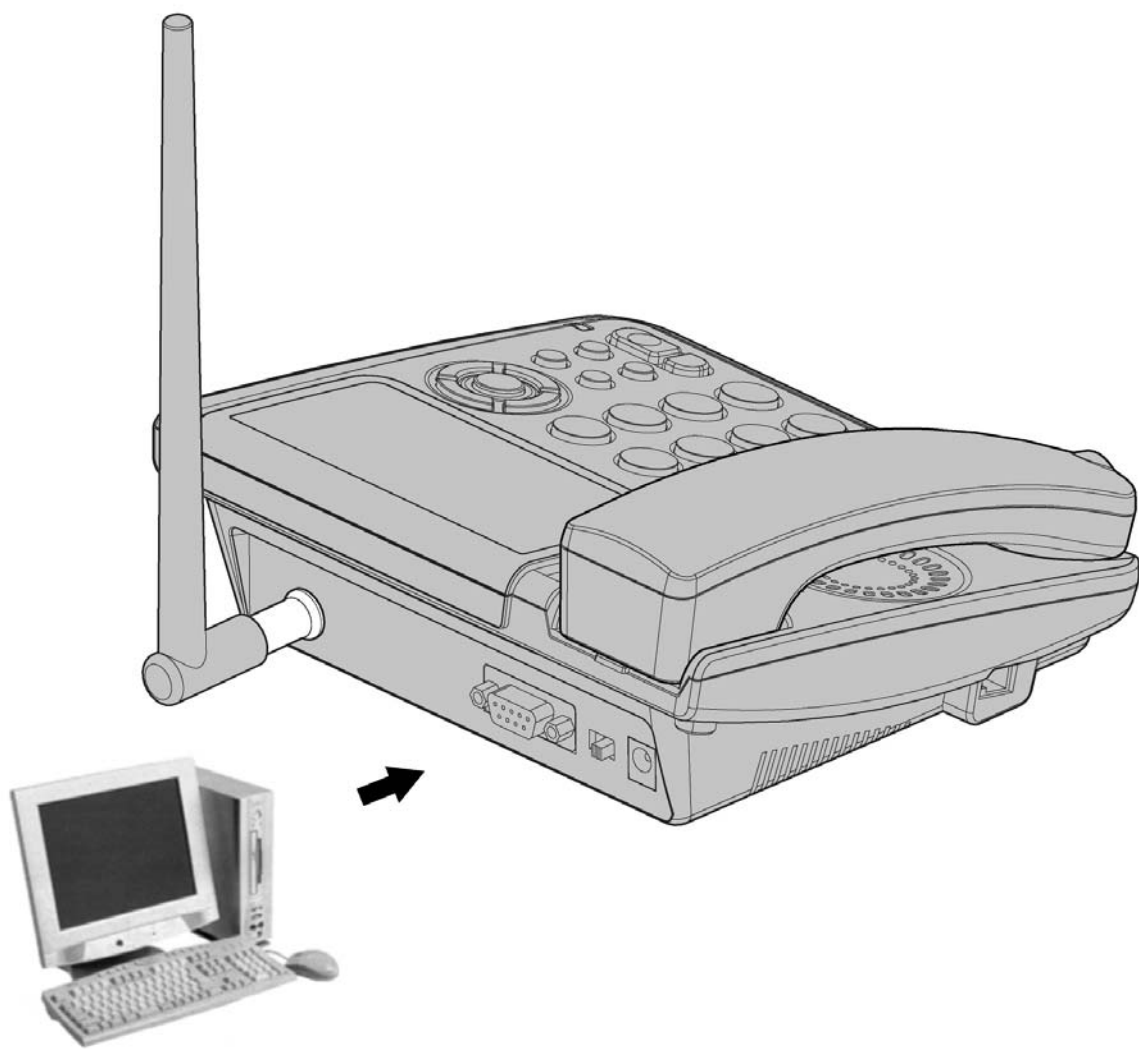
Figure 4-5 Connecting the FWT to a PC through a serial communication cable
