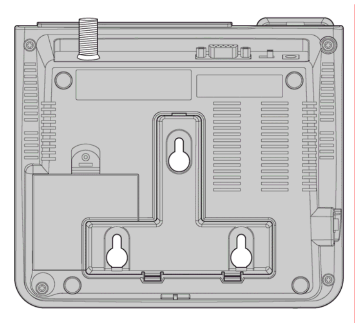
Figure 4-8 Wall-mounting bracket installation
