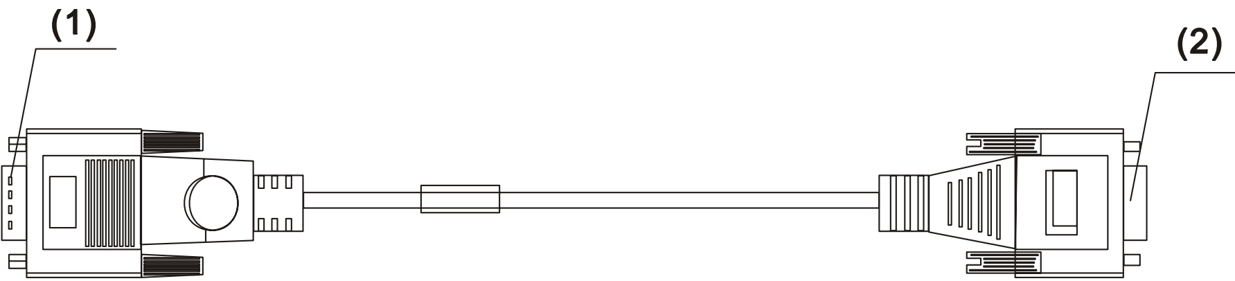
1) Cable connector-D type-9 pin-male 2) Cable connector-D type-9 pin-female Figure 4-4 Serial communication cable
