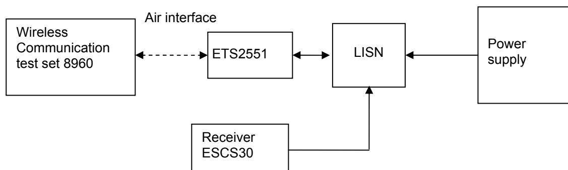
Figure 10. Test Set-up
