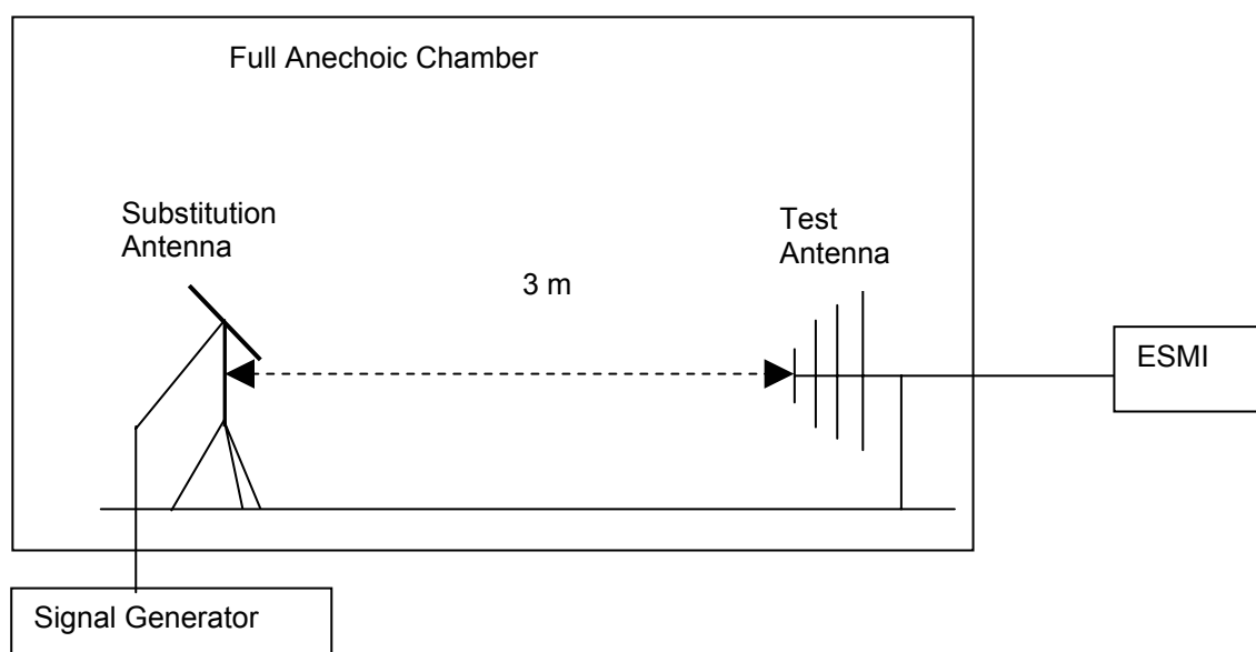
Figure 6. Test Set-up
