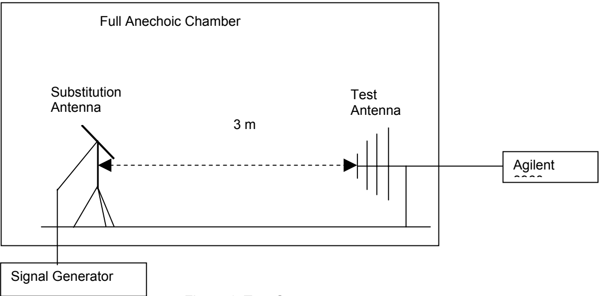
Figure 1. Test Set-up
