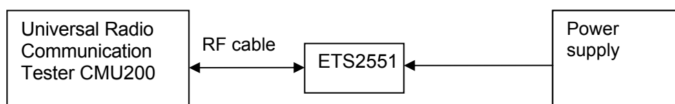
Figure 2. Test Set-up
