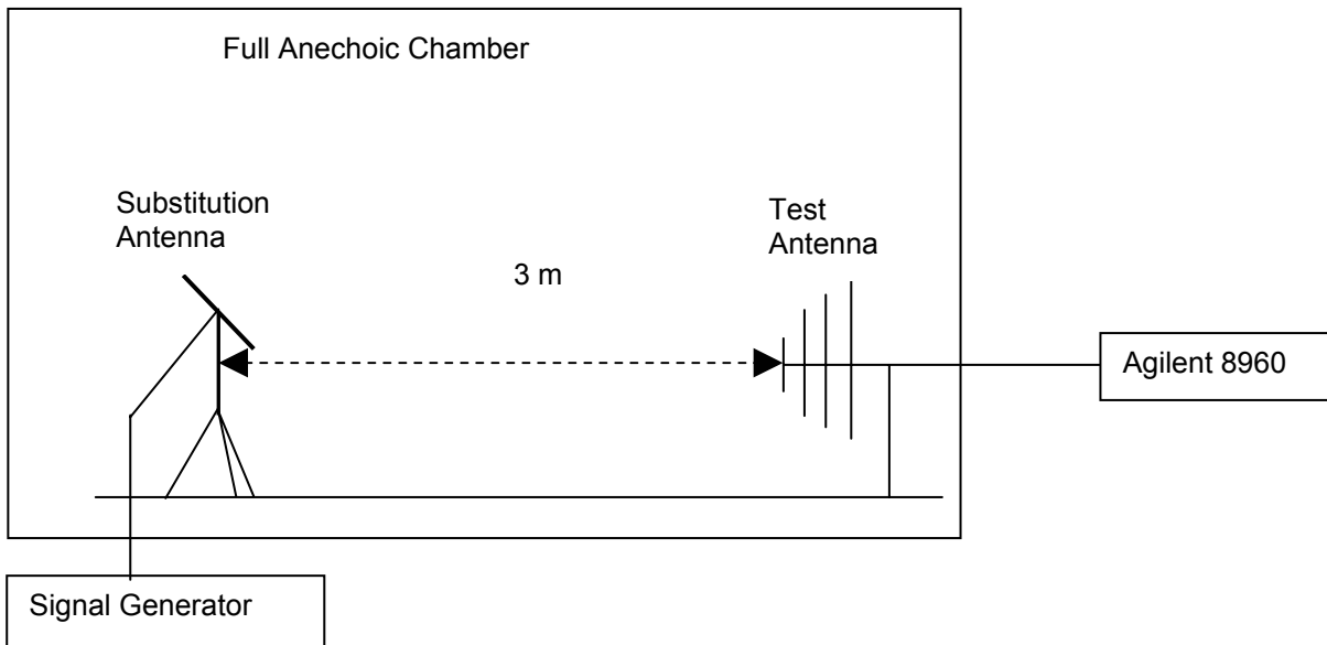
Figure 1. Test Set-up
