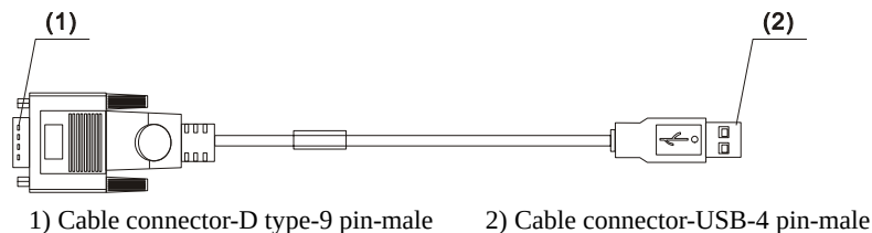
Figure 4-3 USB serial cable
