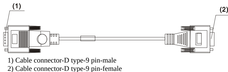
Figure 4-4 Serial communication cable
