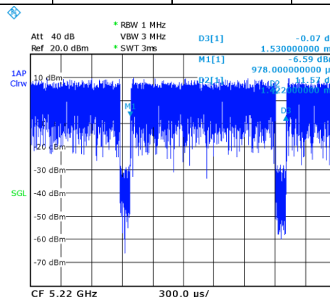
Picture 14.2 The plot of duty factor for UNII-1
