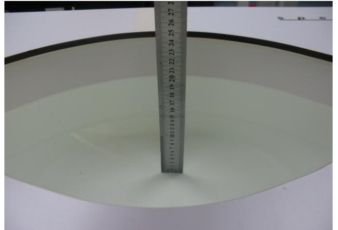
Photo 23: MSL1900MHz depth (15.2cm)
