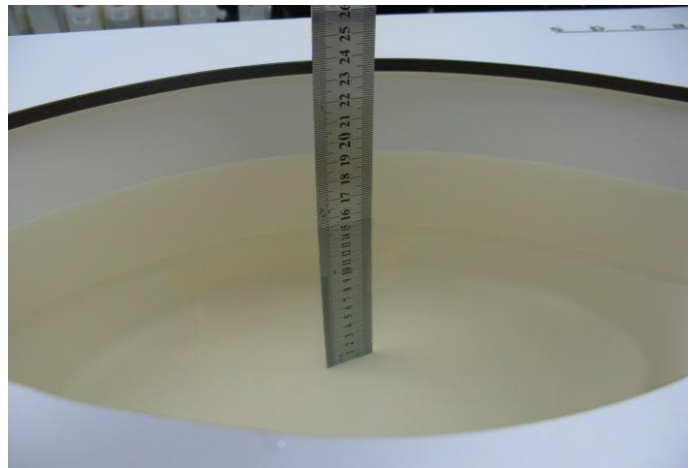
Photo 19: MSL835MHz depth (15.1cm)
