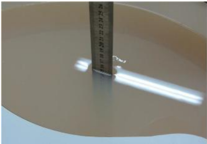
Photo 29:MBBL3500-5800MHz Depth (15.2cm)
