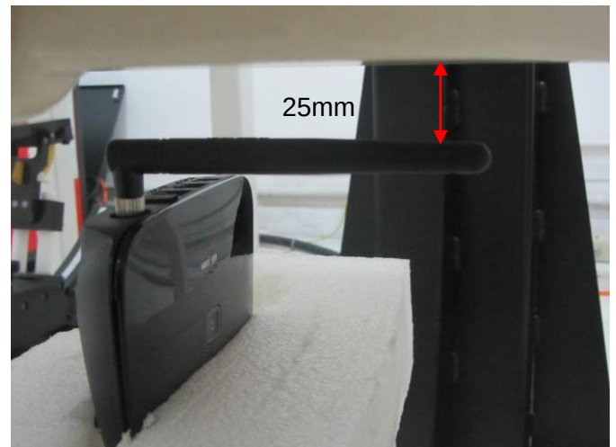
Photo 5: Top side with antenna vertical(25mm)
