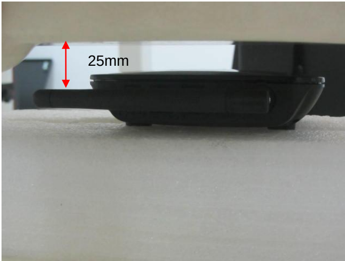
Photo 6: Front side with antenna horizontal (25mm)
