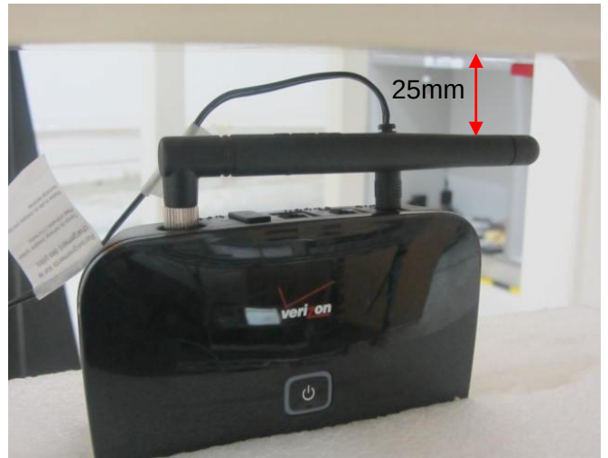
Photo 7: Top side with antenna horizontal with DC Power adapter(25mm)
