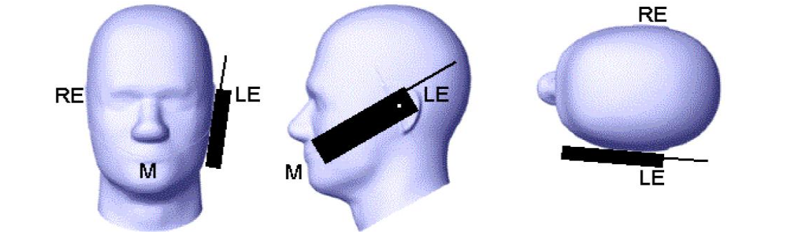
Picture D.2 Cheek position of the wireless device on the left side of SAM
