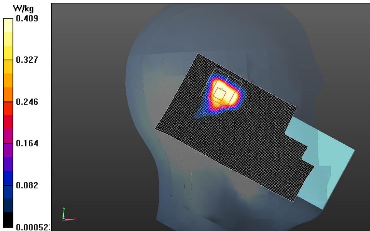
Fig.26 Wi-Fi 2.4G
