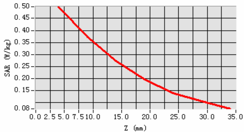
SAR, Z Axis Scan (X = -40, Y = -31)
