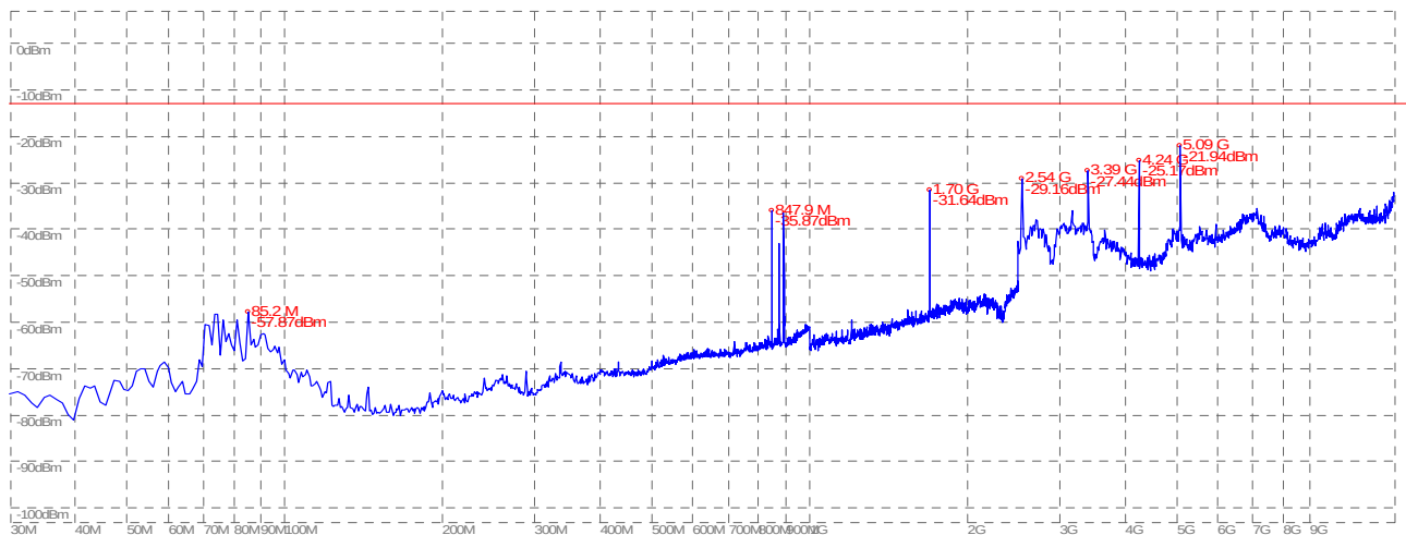
(Plot C.2: GSM 850MHz Channel = 251, Test Antenna Vertical)
