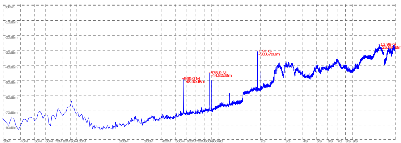
(Plot F.2: GSM 1900MHz Channel = 810, Test Antenna Vertical)
