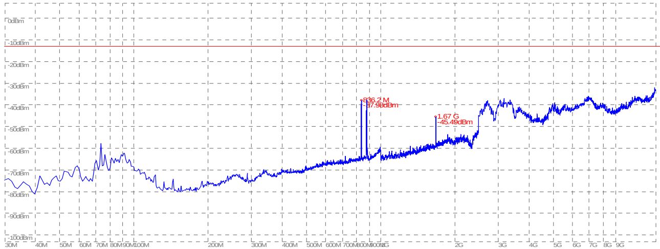
(Plot B.2: GSM 850MHz Channel = 190, Test Antenna Vertical)
