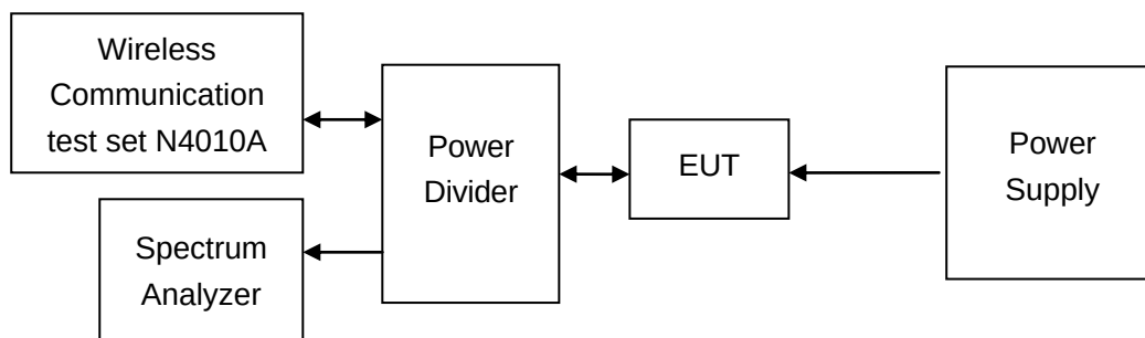
Figure 7. Test Set-up
