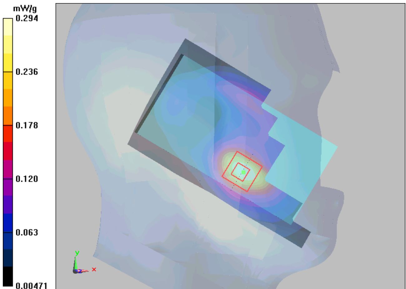
Figure 29 Left Hand Touch Cheek GSM 1900 Channel 661
