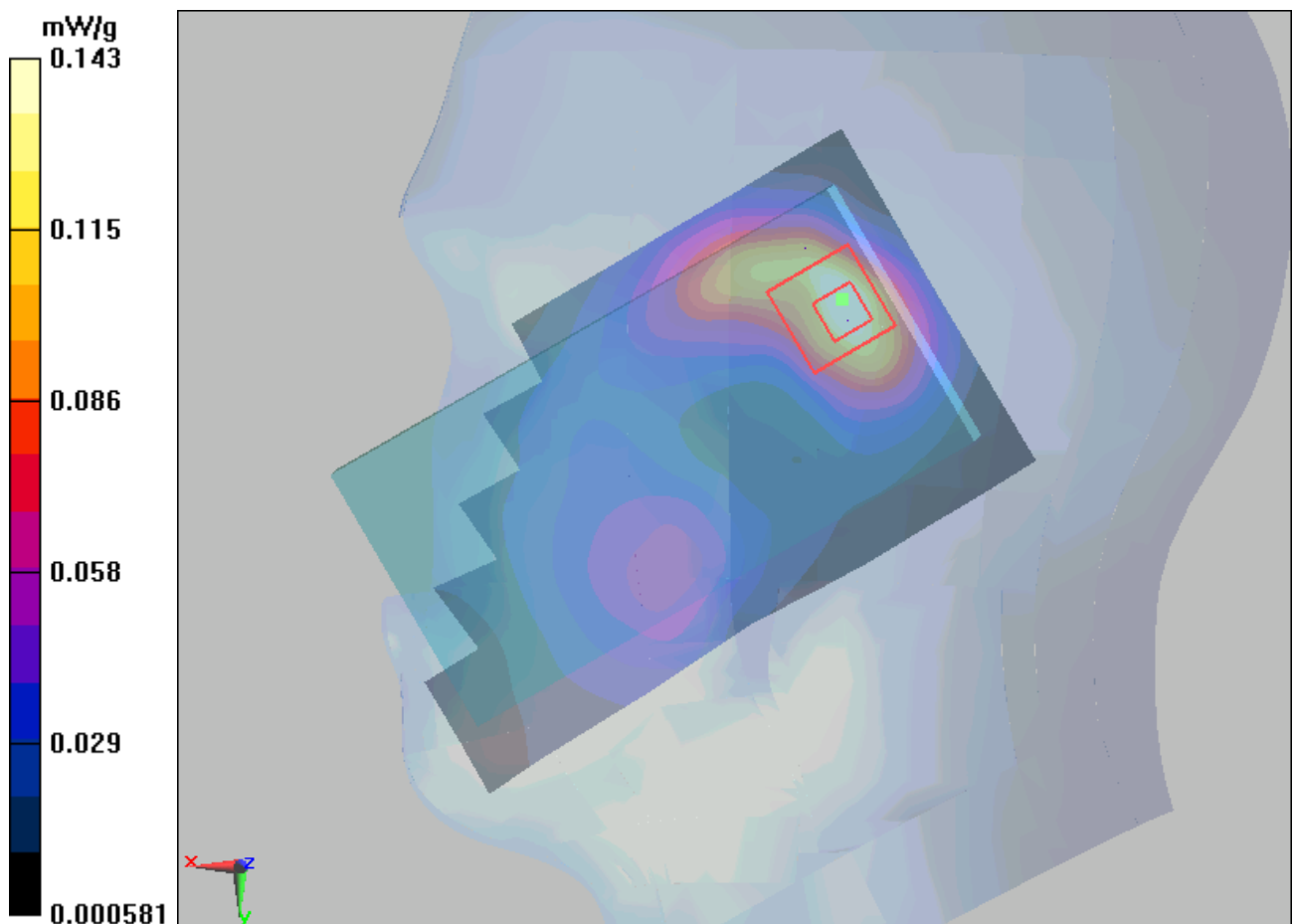
Figure 32 Right Hand Tilt 15° GSM 1900 Channel 661
