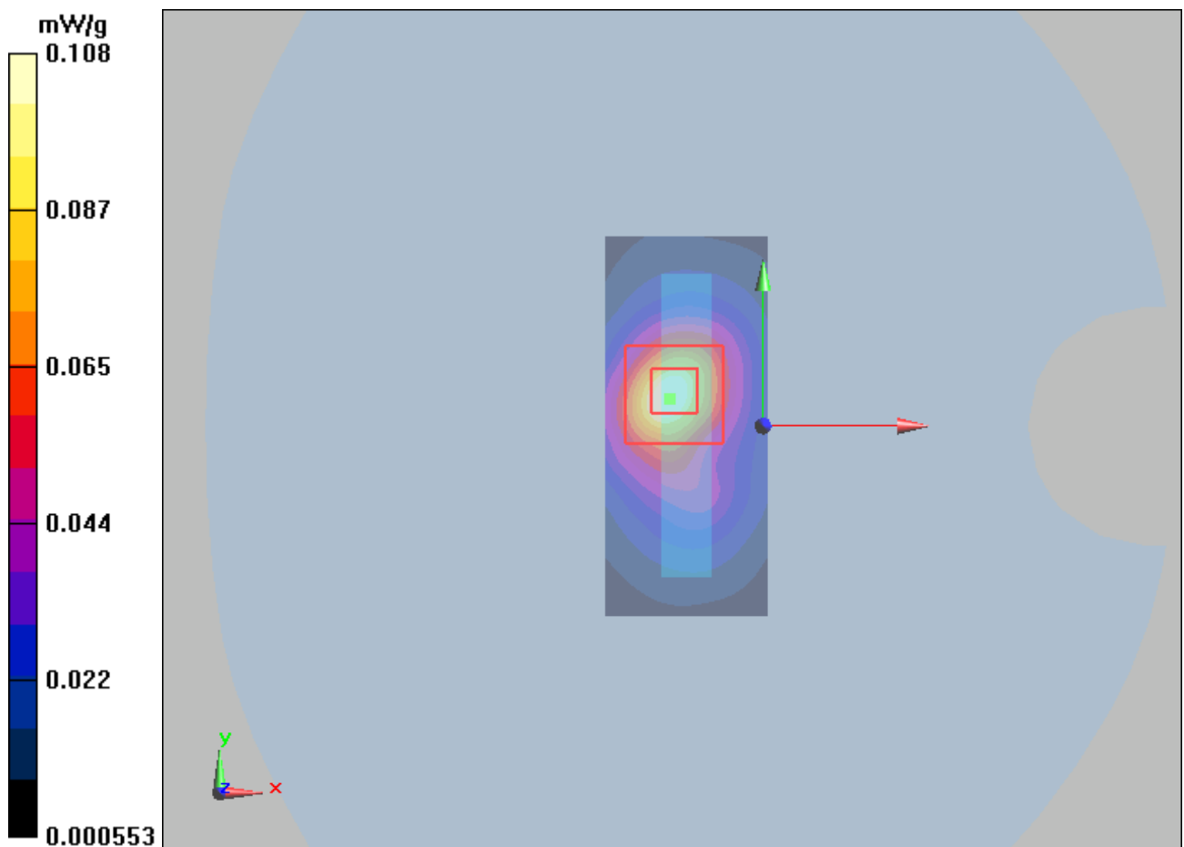
Figure 54 Body, Top Edge, 802.11b Channel 11
