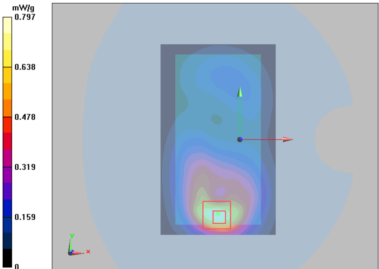
Figure 40 Body, Back Side, GSM 1900 EGPRS (2Txslots) Channel 661
