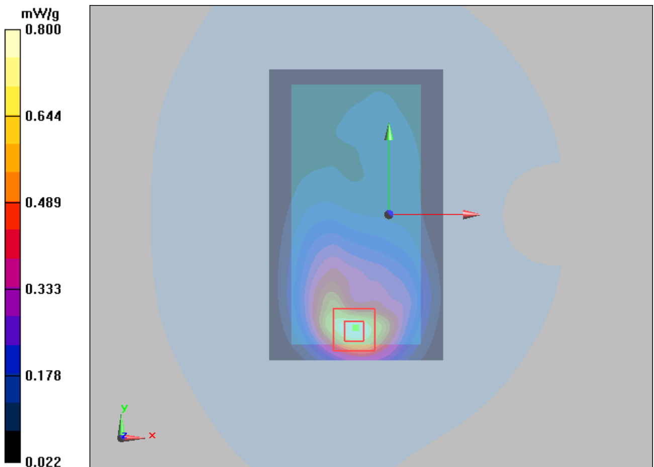
Figure 41 Body with Earphone, Back Side, GSM 1900 Channel 661
