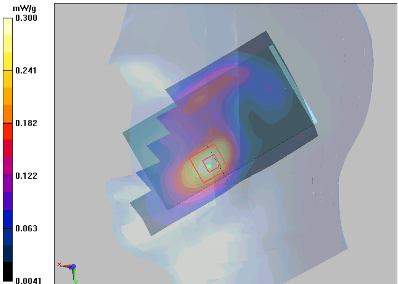
Figure 31 Right Hand Touch Cheek GSM 1900 Channel 661
