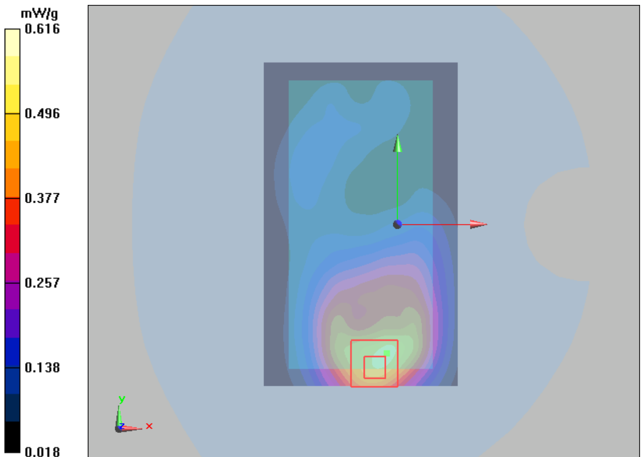
Figure 36 Body, Front Side, GSM 1900 GPRS (2Txslots) Channel 661
