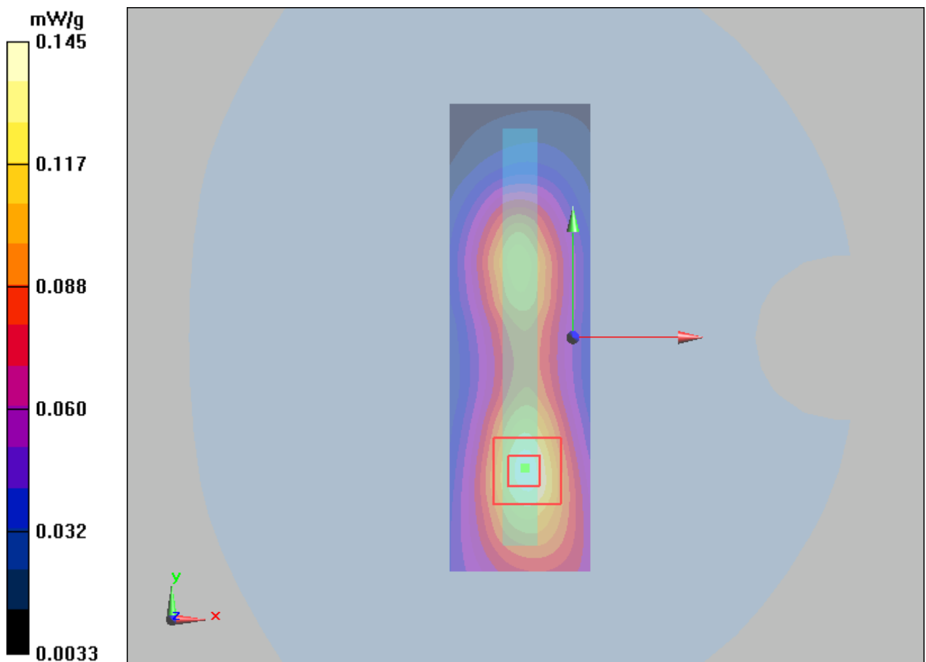
Figure 38 Body, Right Edge, GSM 1900 GPRS (2Txslots) Channel 661
