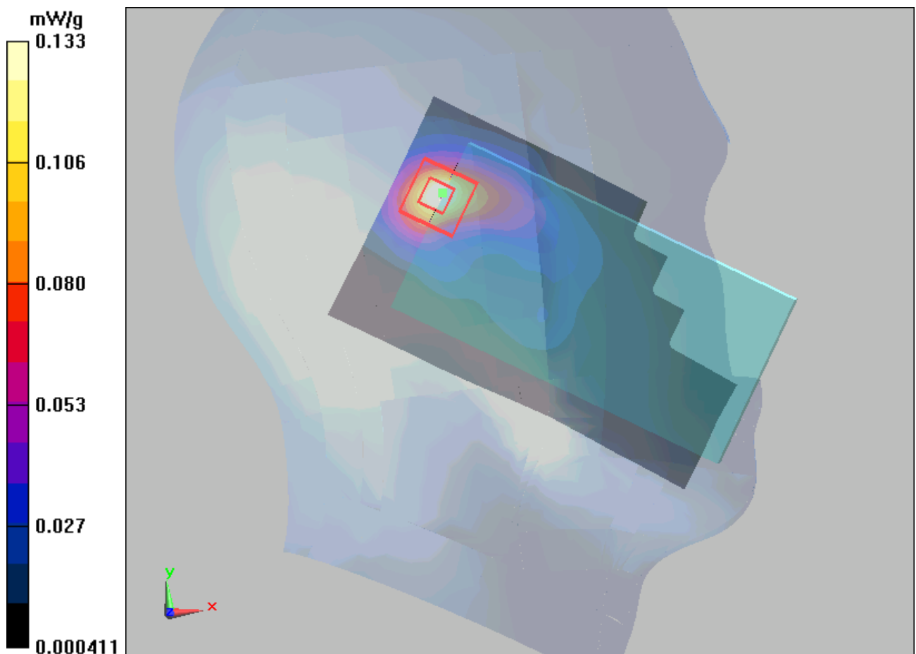
Figure 45 Left Hand Touch Cheek 802.11b Channel 11
