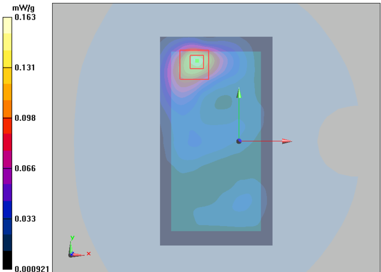
Figure 50 Body, Back Side, 802.11b Channel 11
