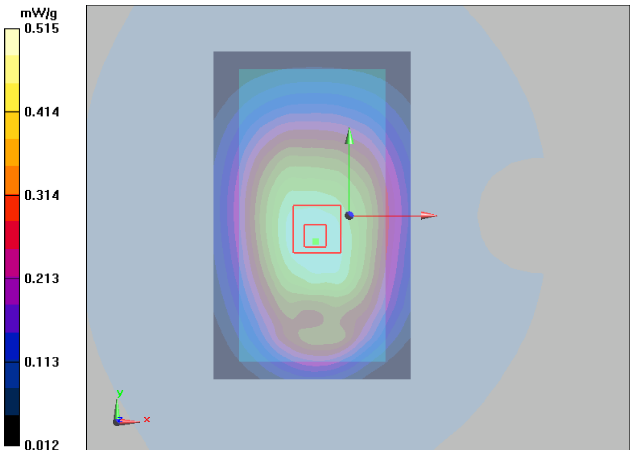
Figure 28 Body, Back Side, GSM 850 GPRS (2Txslots) Channel 190
