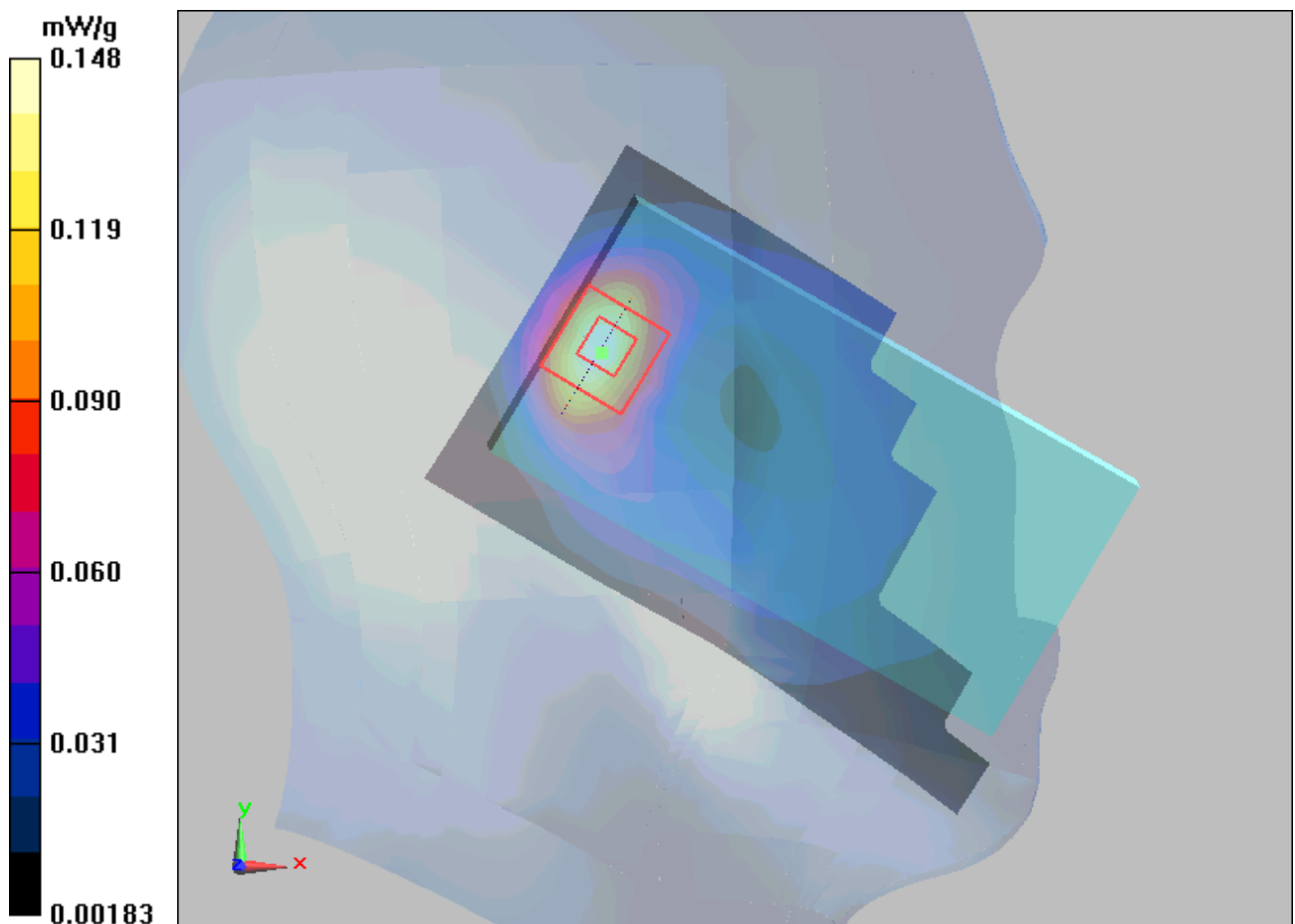
Figure 30 Left Hand Tilt 15° GSM 1900 Channel 661
