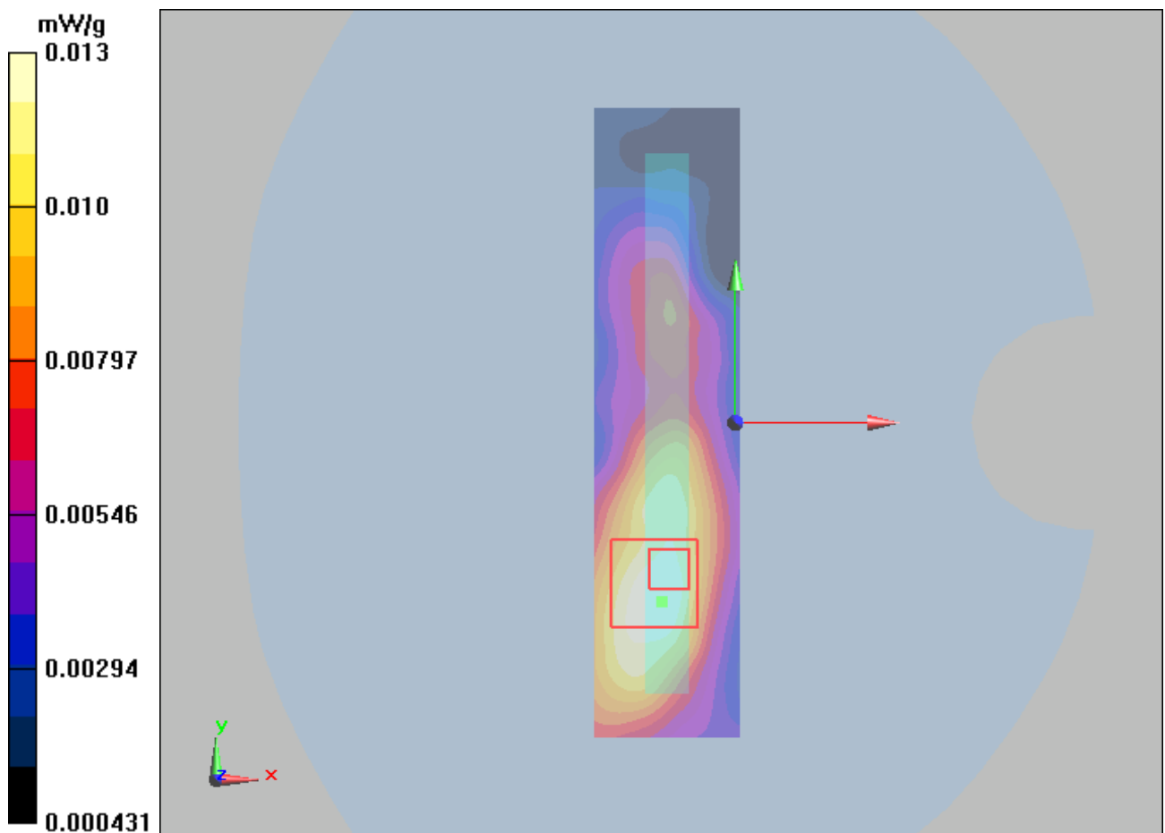
Figure 53 Body, Right Edge, 802.11b Channel 11
