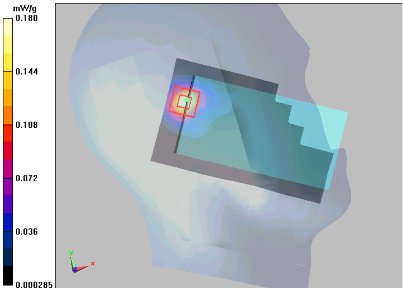
Figure 49 Left Hand Tilt 15° 802.11b Channel 11
