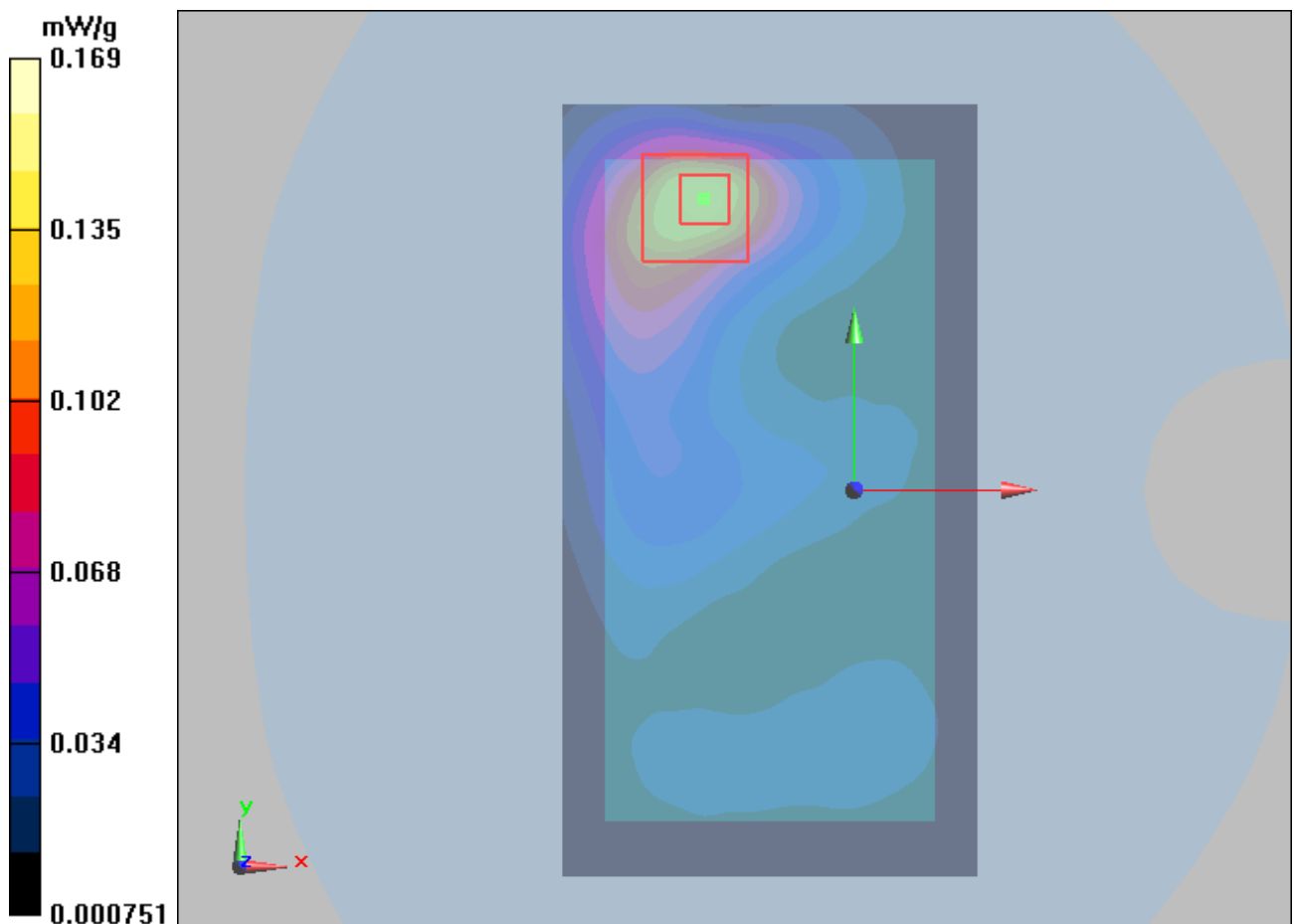
Figure 58 Body with Earphone, Back Side, 802.11b Channel 11
