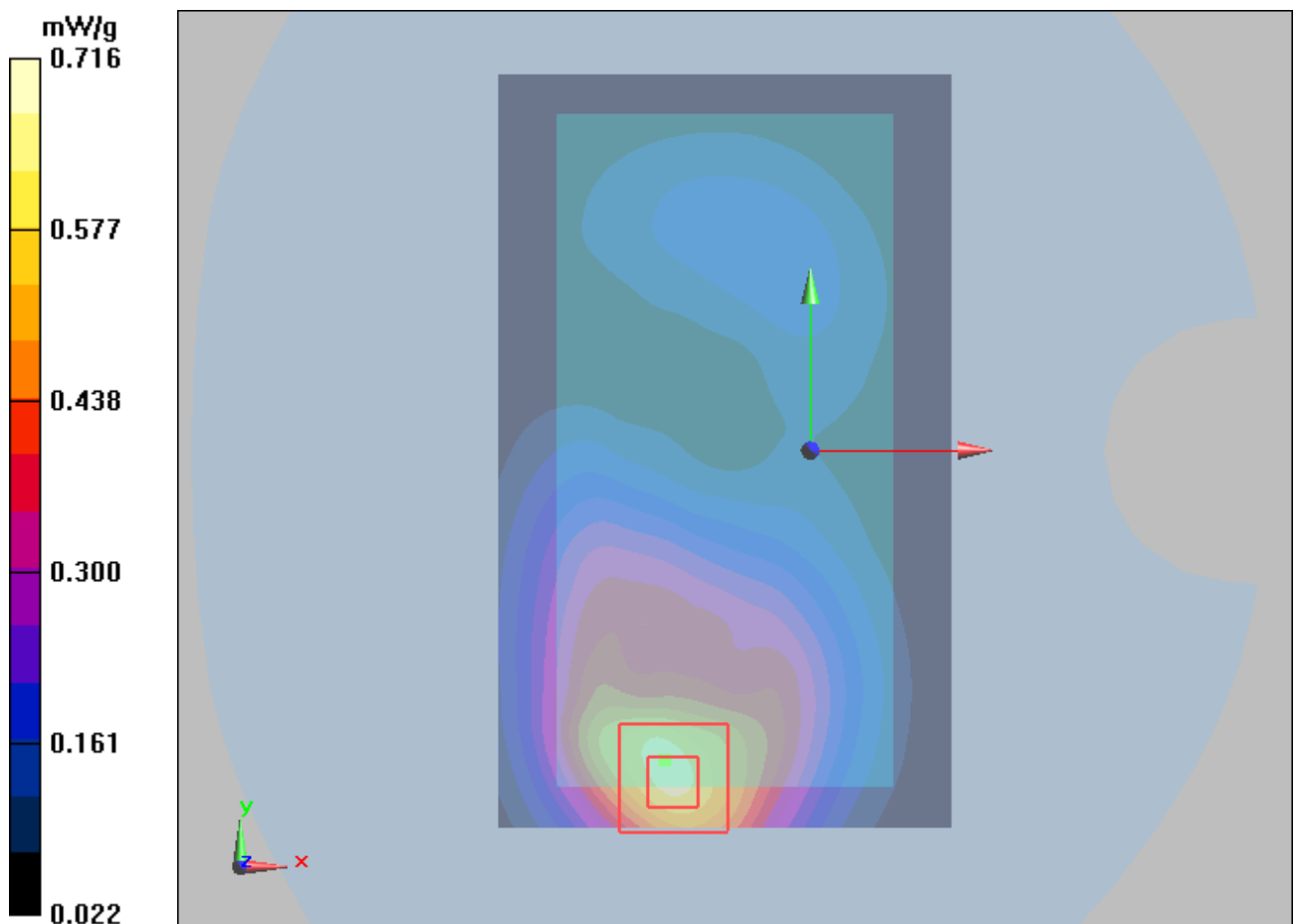
Figure 44 Body, Back Side, GSM 1900 GPRS (2Txslots) Channel 661
