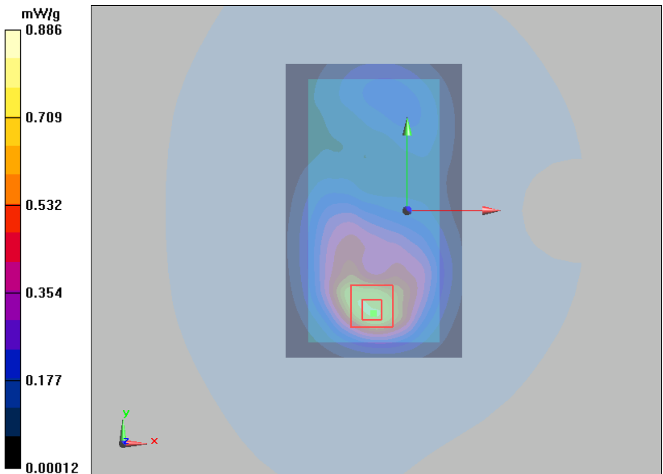
Figure 42 Body, Back Side, GSM 1900 GPRS (2Txslots) Channel 661
