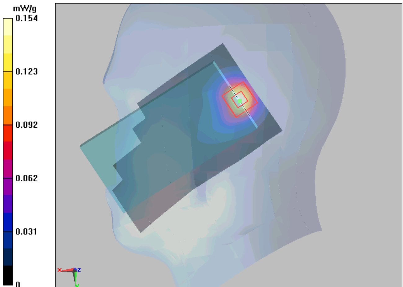
Figure 48 Right Hand Tilt 15° 802.11b Channel 11
