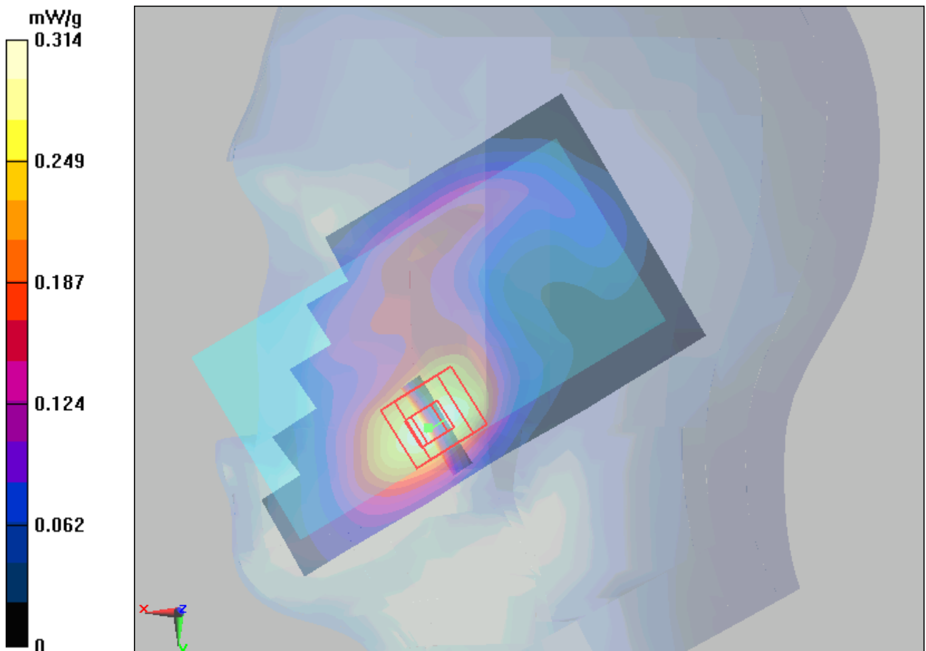
Figure 43 Right Hand Touch Cheek GSM 1900 Channel 661
