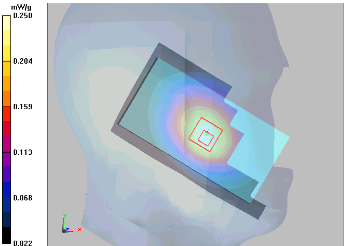
Figure 27 Left Hand Touch Cheek GSM 850 Channel 190
