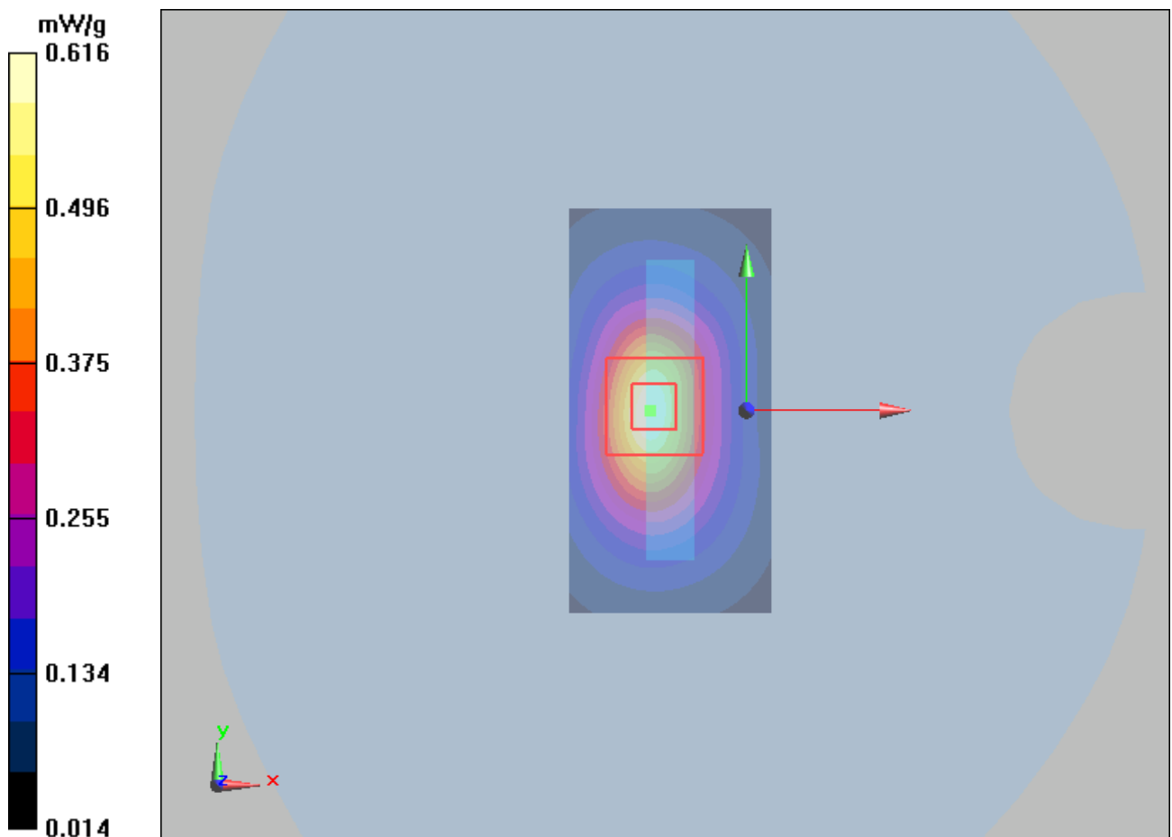
Figure 39 Body, Bottom Edge, GSM 1900 GPRS (2Txslots) Channel 661
