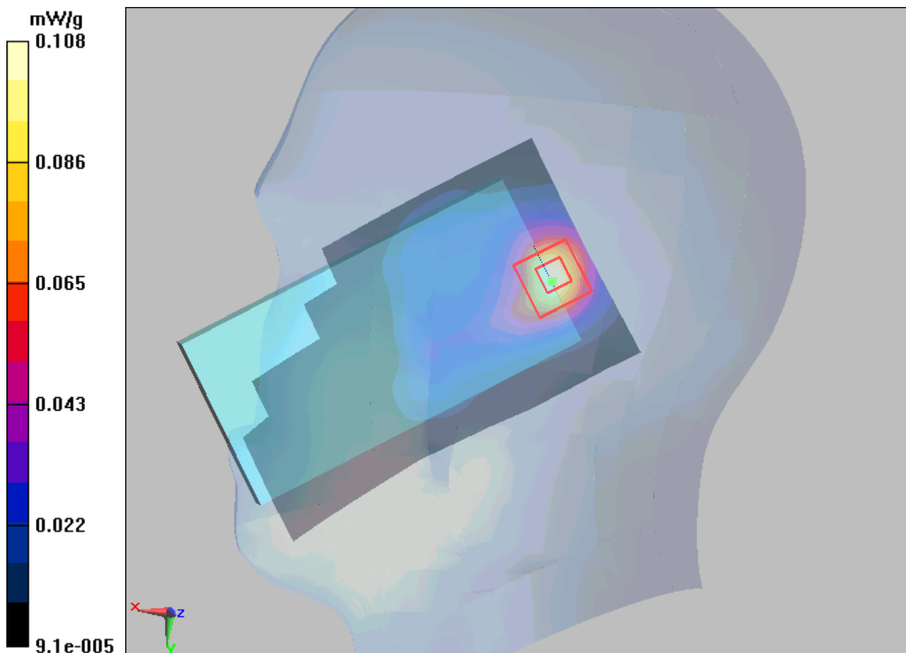
Figure 47 Right Hand Touch Cheek 802.11b Channel 11
