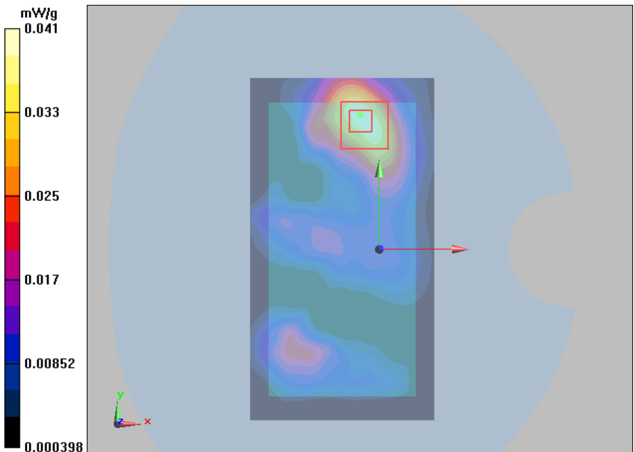
Figure 51 Body, Front Side, 802.11b Channel 11
