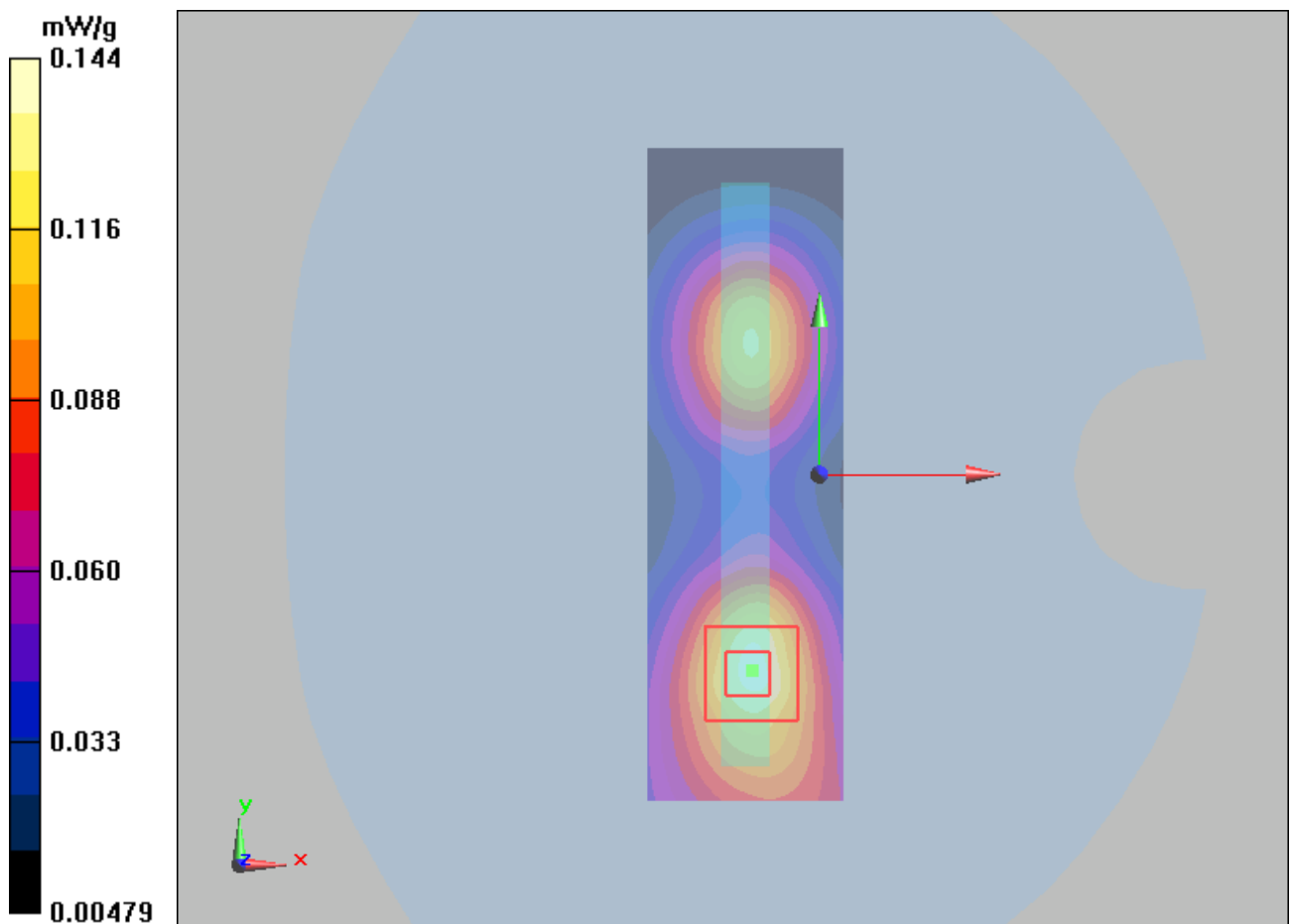
Figure 37 Body, Left Edge, GSM 1900 GPRS (2Txslots) Channel 661
