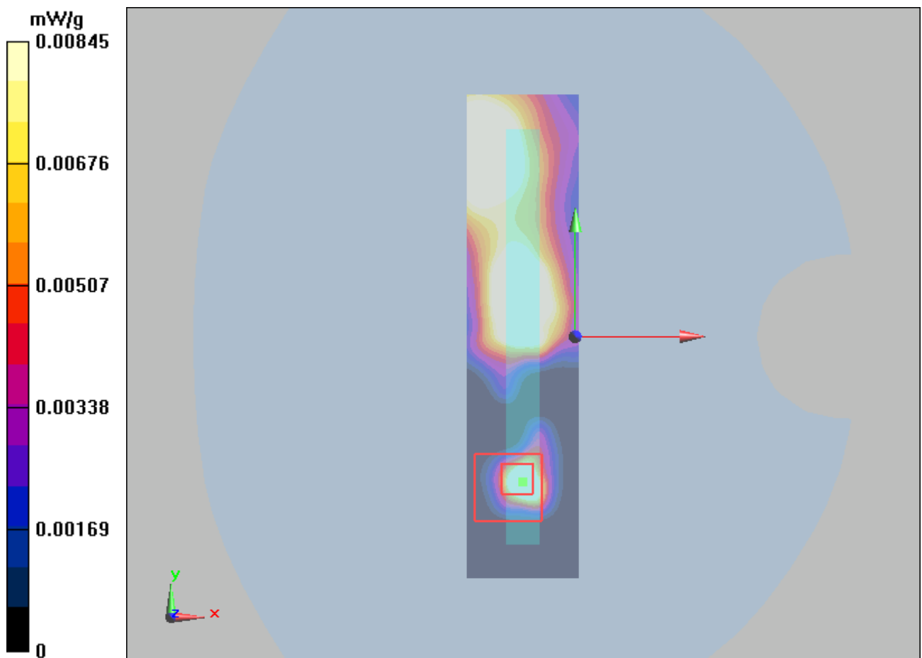
Figure 52 Body, Left Edge, 802.11b Channel 11
