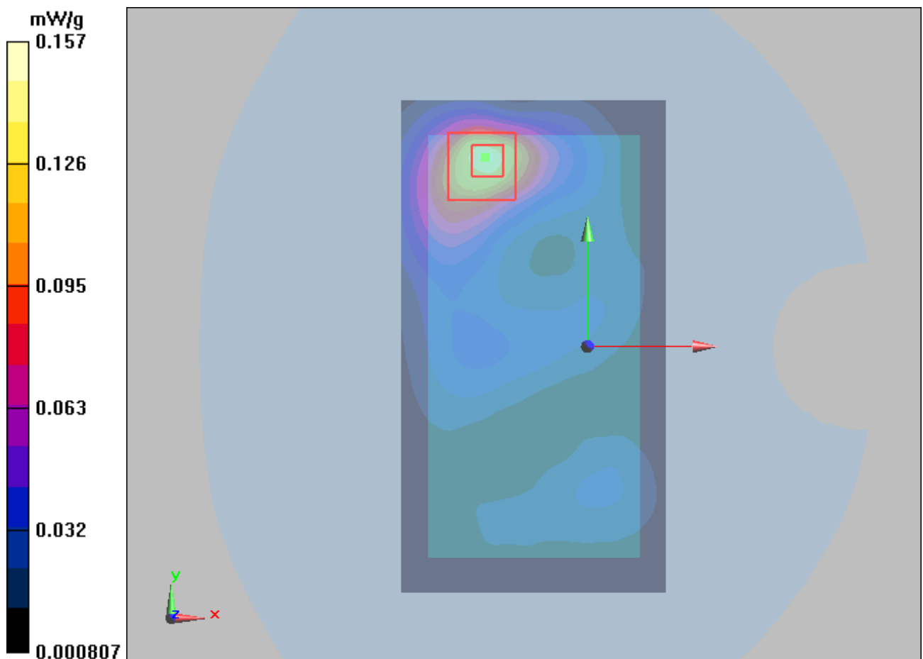
Figure 56 Body, Back Side, 802.11b Channel 11
