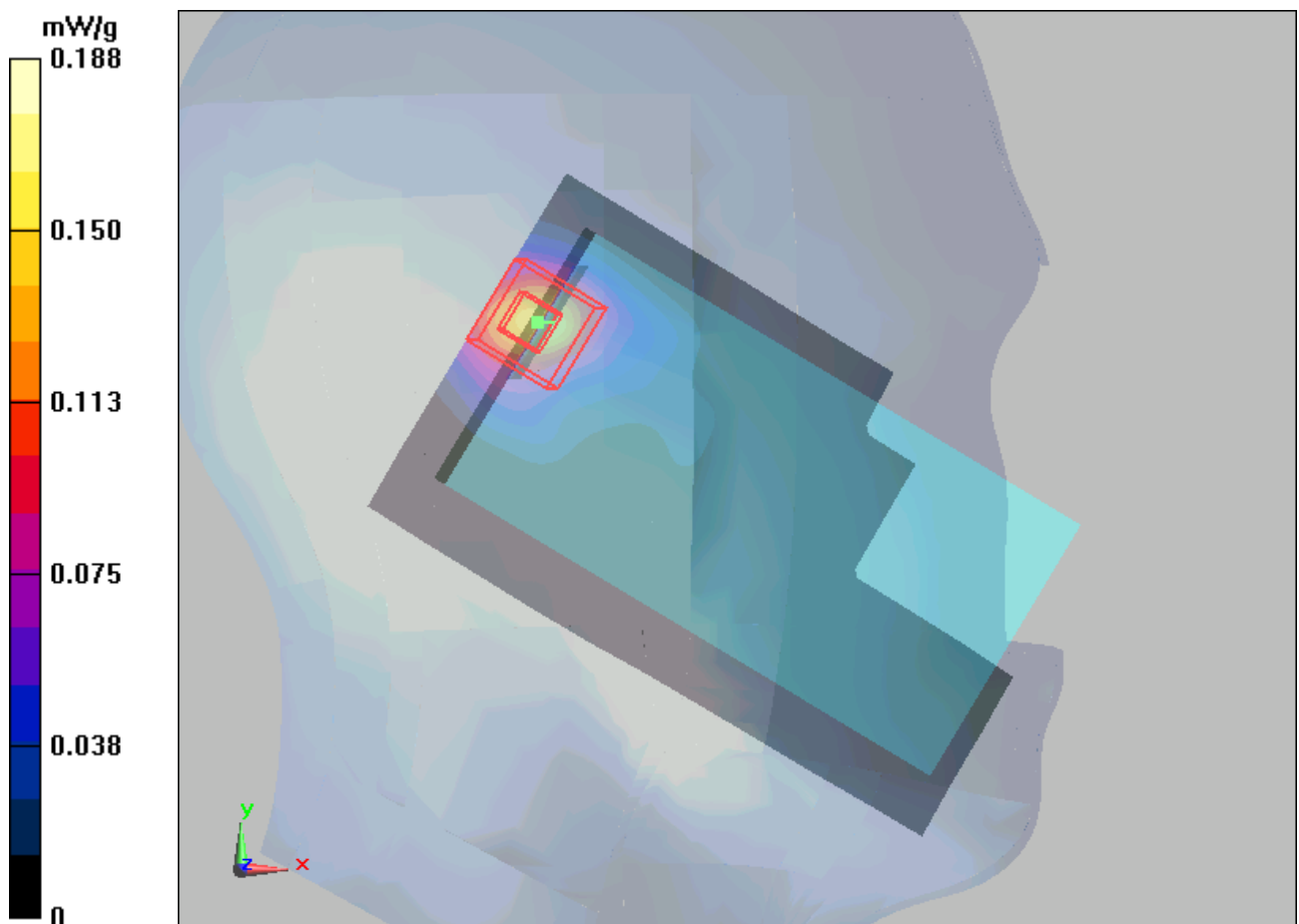
Figure 57 Left Hand Tilt 15° 802.11b Channel 11
