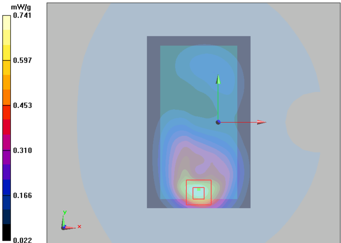
Figure 34 Body, Back Side, GSM 1900 GPRS (1Txslot) Channel 661
