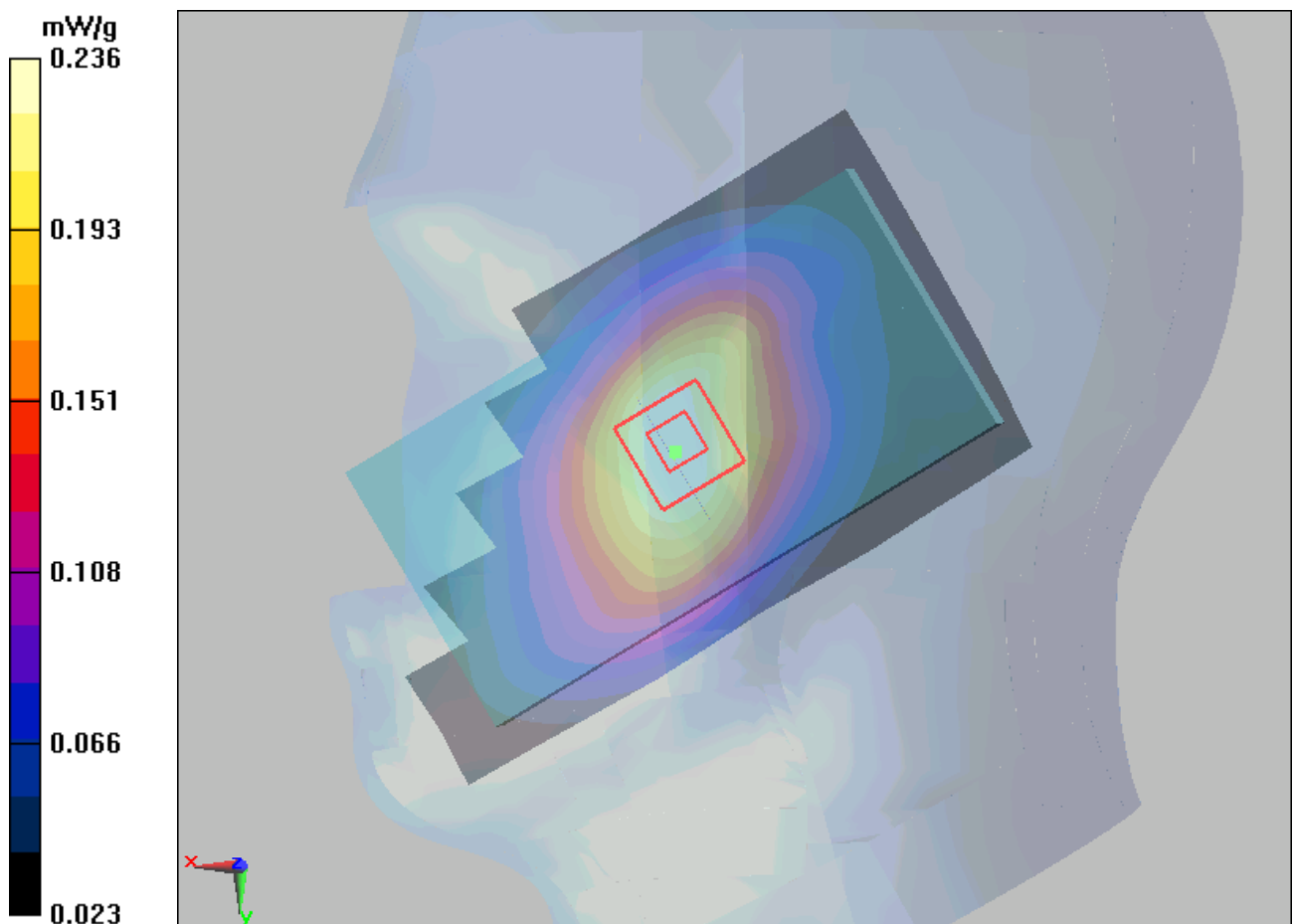
Figure 15 Right Hand Touch Cheek GSM 850 Channel 190
