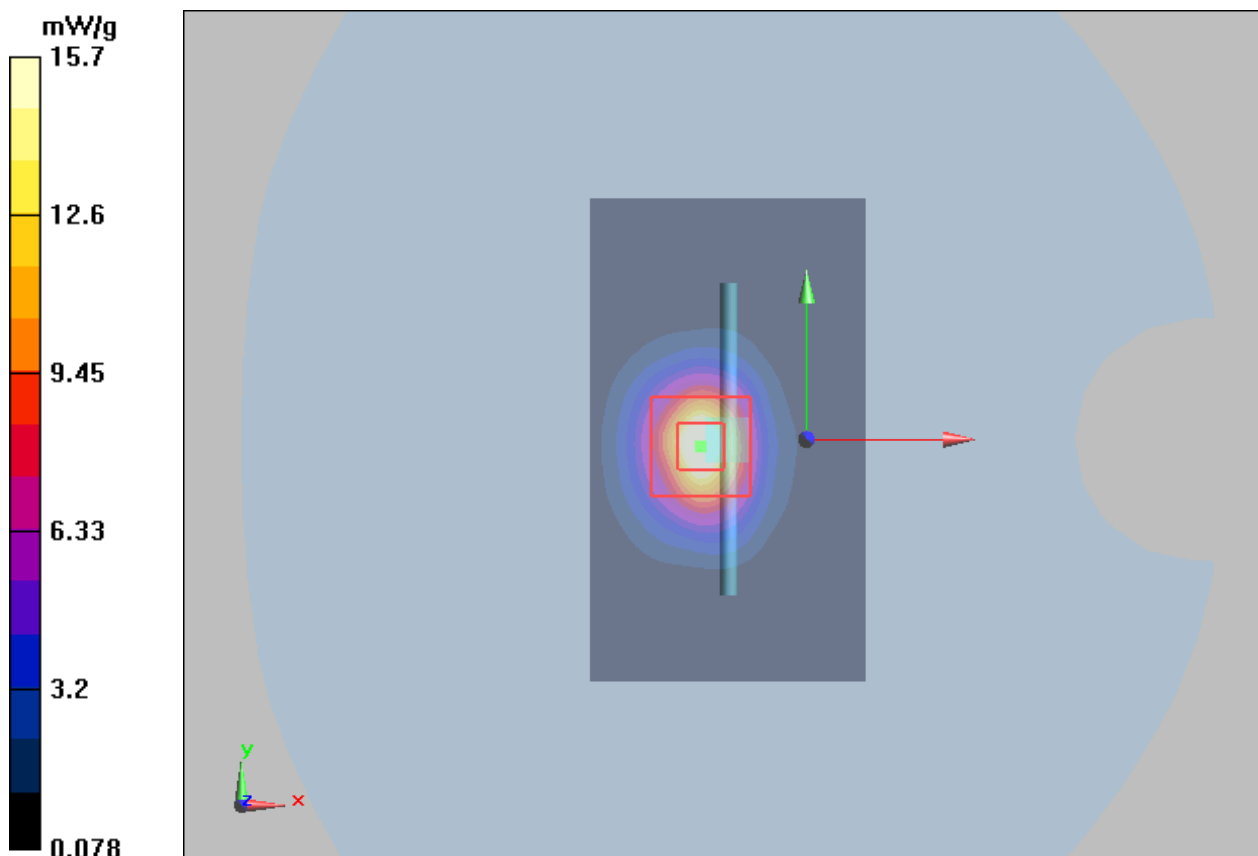
Figure 15 System Performance Check 1900MHz 250mW
