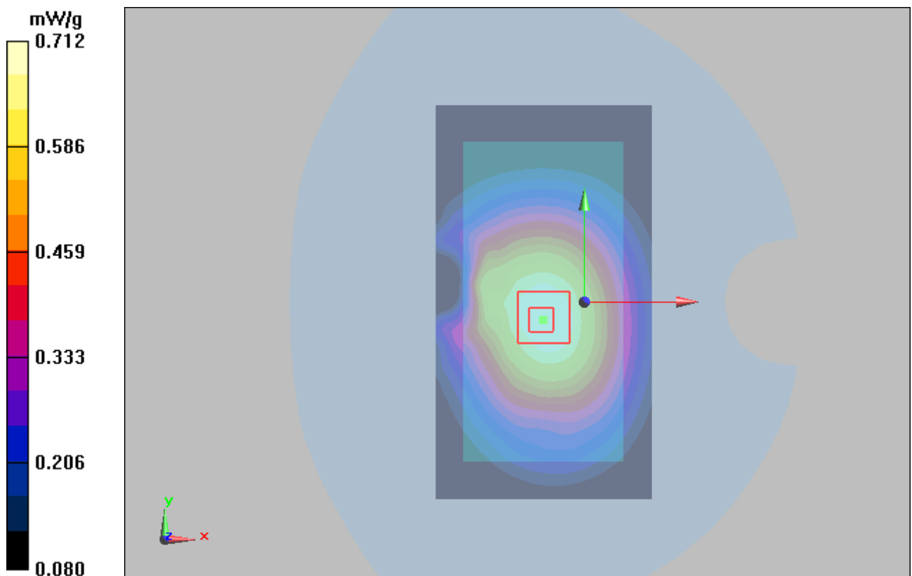
Figure 22 Body, Back Side, GSM 850 GPRS (2Txslots) Channel 251
