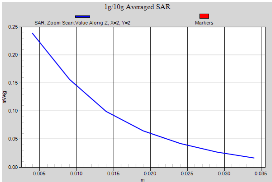
Figure 36 Right Hand Touch Cheek GSM 1900 Channel 661
