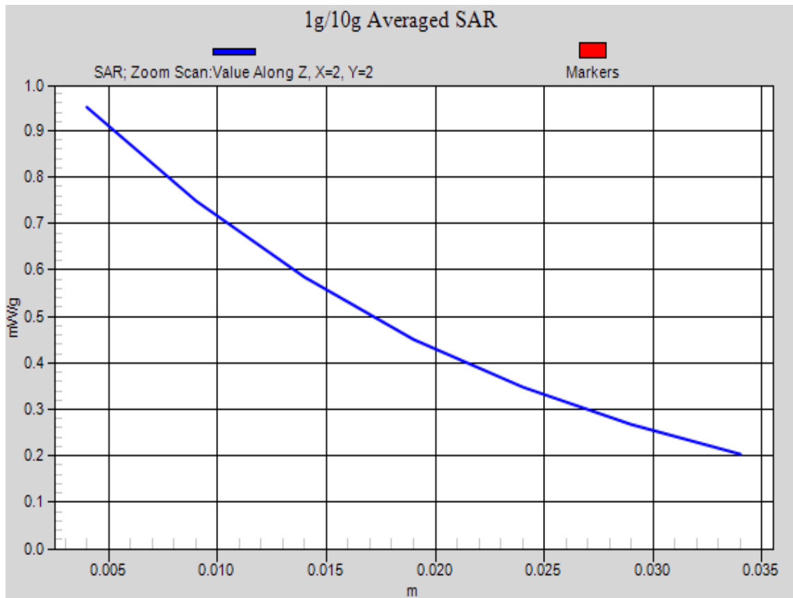
Figure 60 Body, Back Side, WCDMA Band V Channel 4233
