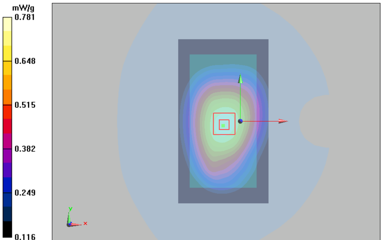
Figure 65 Body, Front Side, WCDMA Band V Channel 4132
