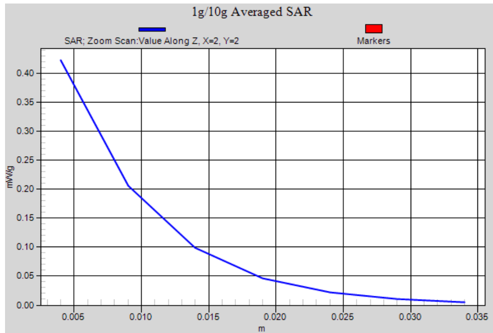
Figure 88 Left Hand Touch Cheek 802.11b Channel 6
