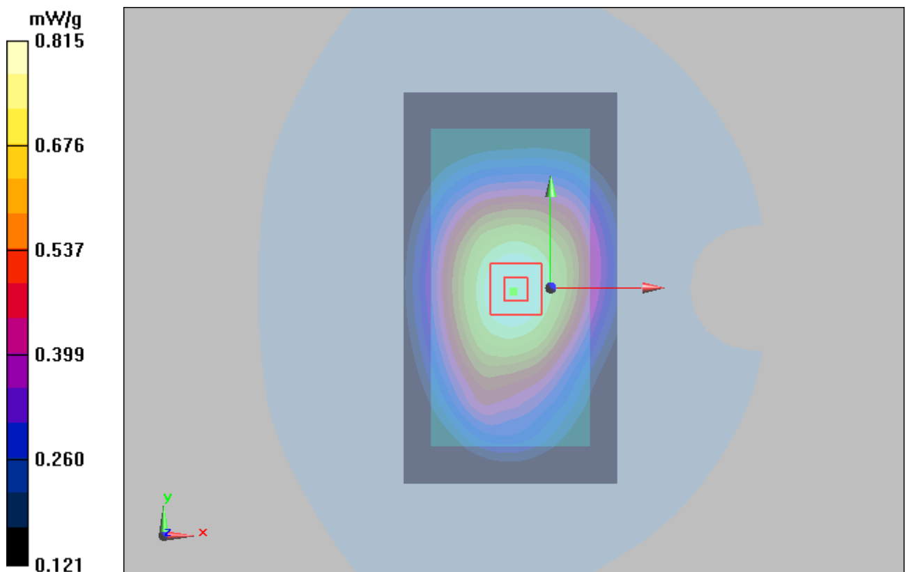
Figure 63 Body, Front Side, WCDMA Band V Channel 4233
