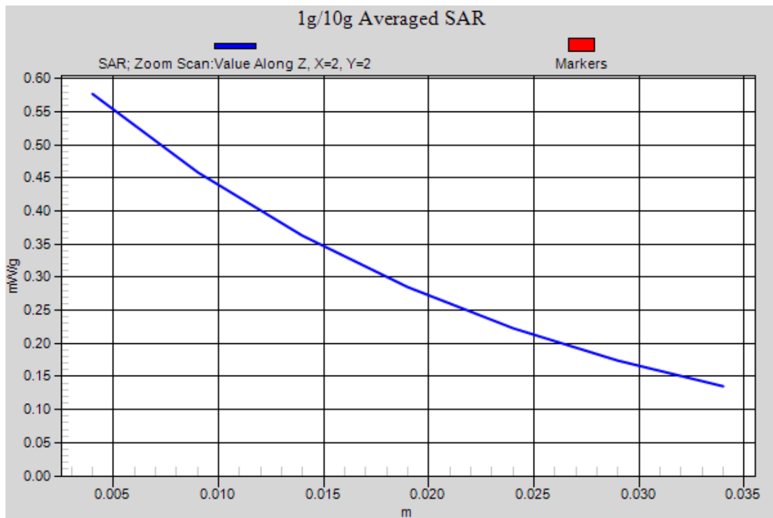
Figure 52 Right Hand Touch Cheek WCDMA Band V Channel 4183
