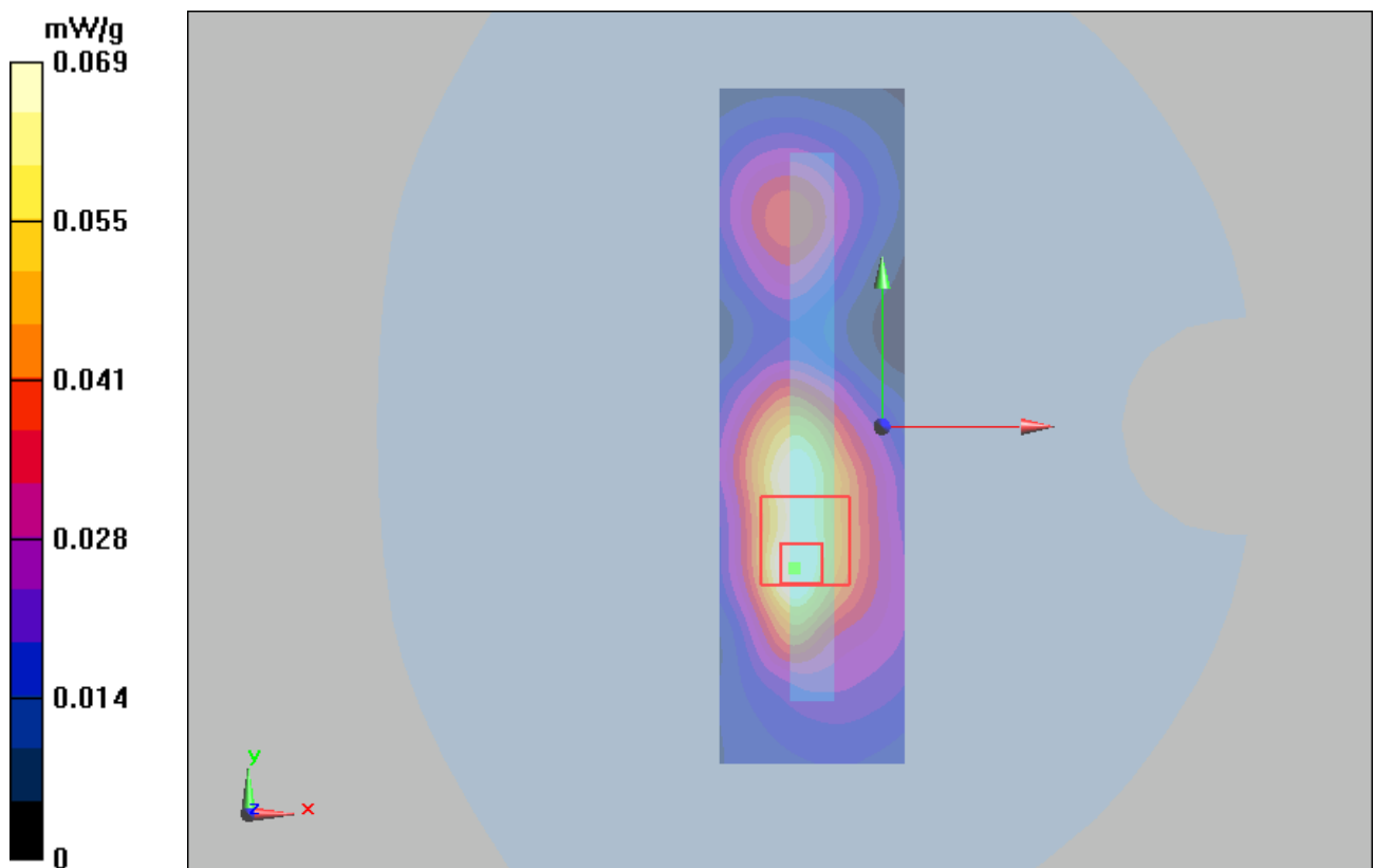
Figure 96 Body, Right Edge, 802.11b Channel 6
