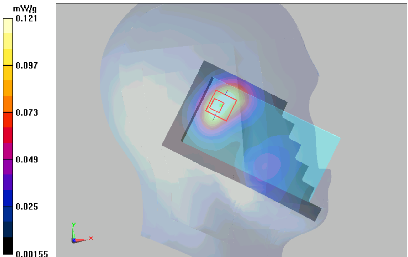
Figure 35 Left Hand Tilt 15° GSM 1900 Channel 661
