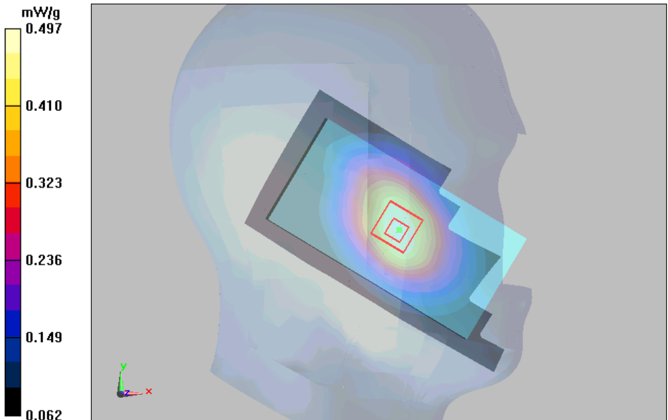
Figure 16 Left Hand Touch Cheek GSM 850 Channel 190
