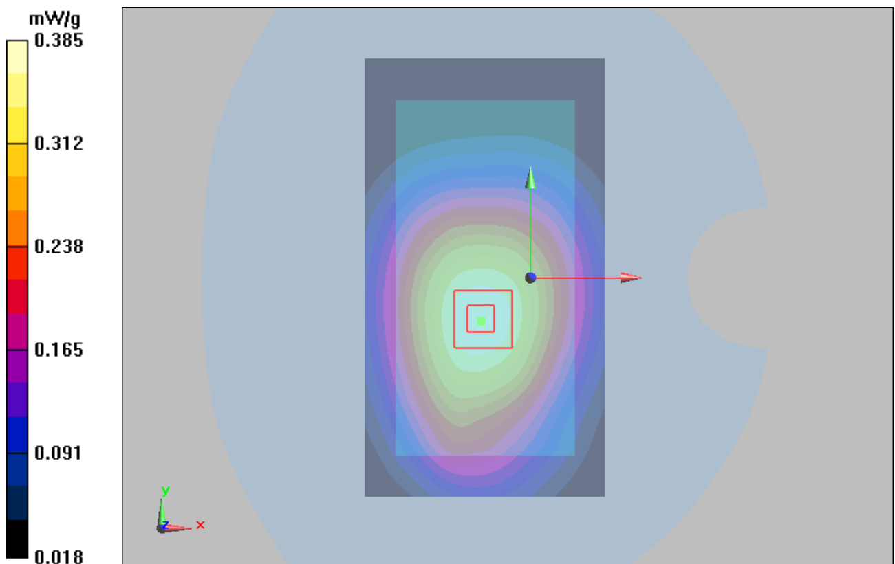
Figure 27 Body, Front Side, GSM 850 GPRS (1 Txslot) Channel 190
