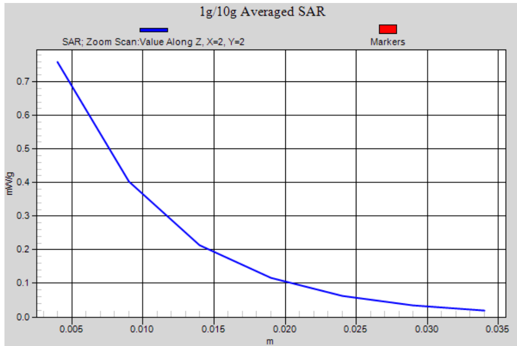
Figure 72 Body, Back Side, LTE Band 7 Channel 21100
