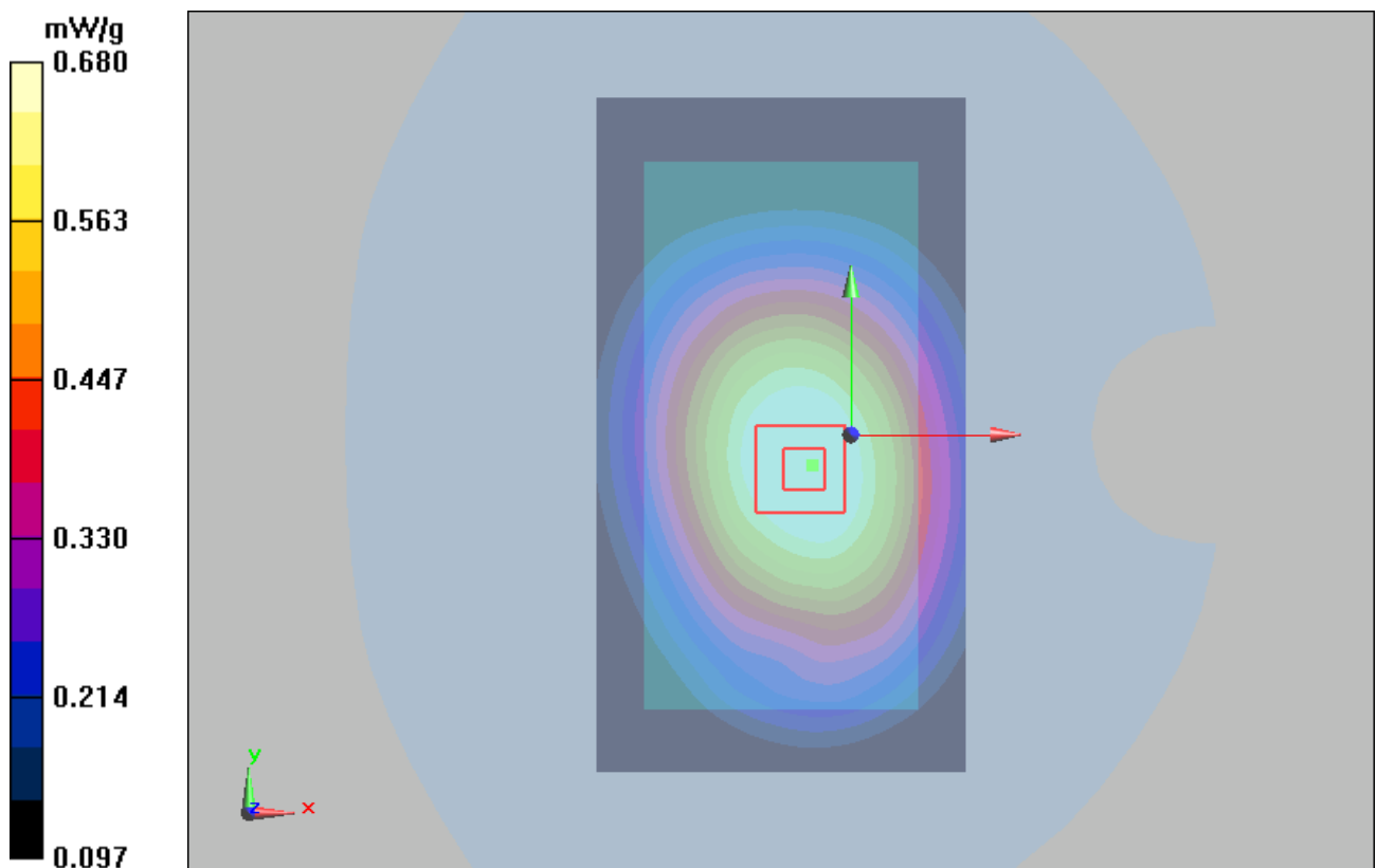
Figure 31 Body, Back Side, GSM 850 EGPRS (2Txslots) Channel 128
