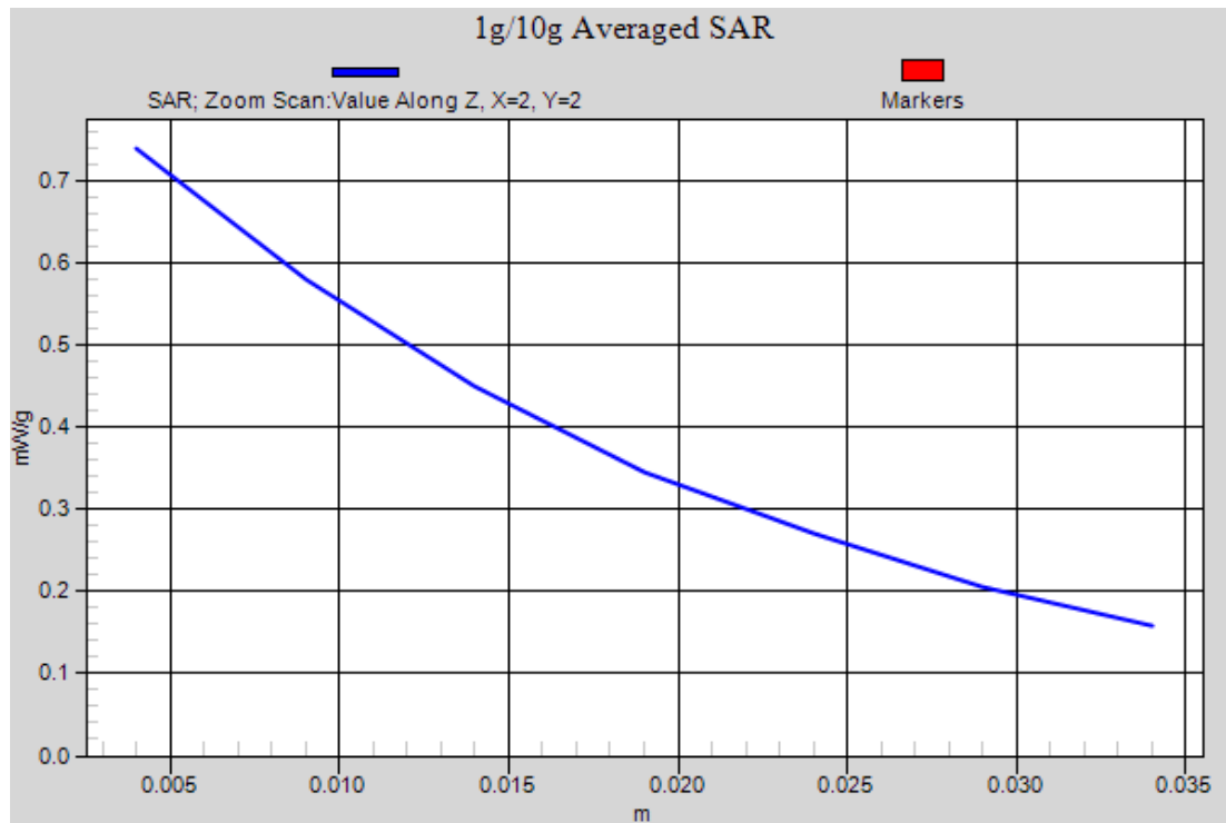
Figure 24 Body, Back Side, GSM 850 GPRS (2Txslots) Channel 128
