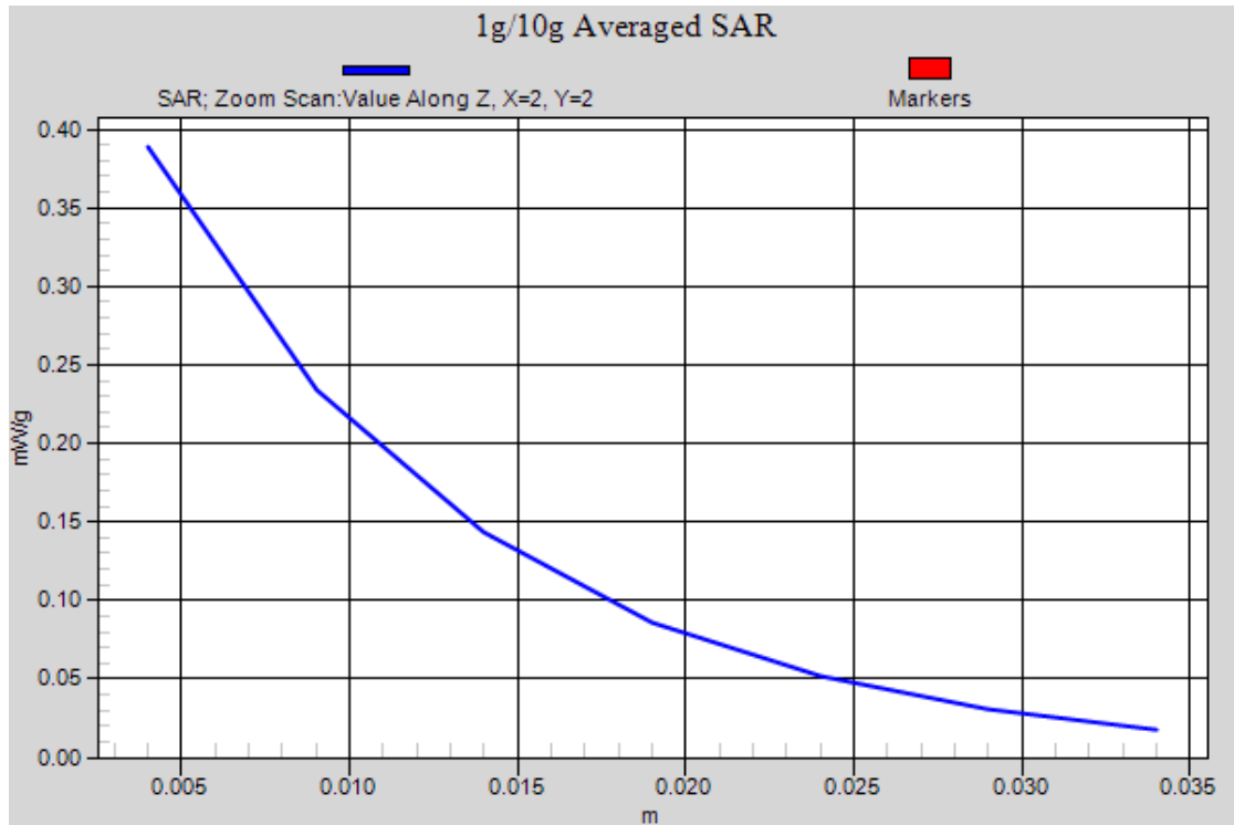
Figure 47 Body, Front Side, GSM 1900 EGPRS (1Txslot) Channel 661
