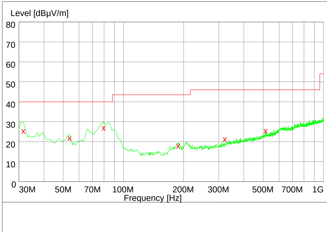
MEASUREMENT RESULT: QP Detector
