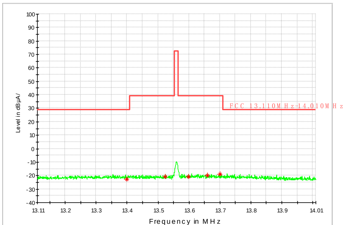
FCC Loop Antenna 13.110MHz-14.010MHz
