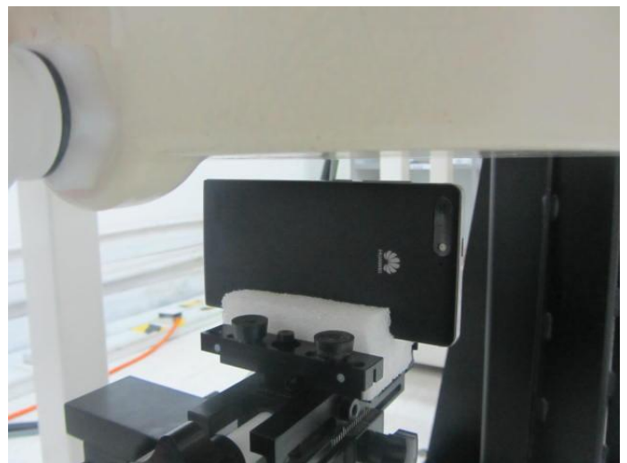
Photo 13: Right Side(10mm)
