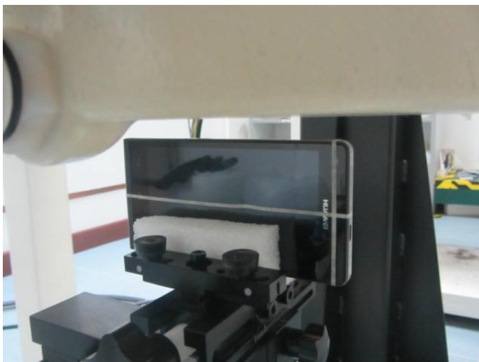
Photo 12:Left Side(10mm)
