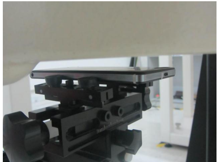
Photo 13: Right Side(10mm)
