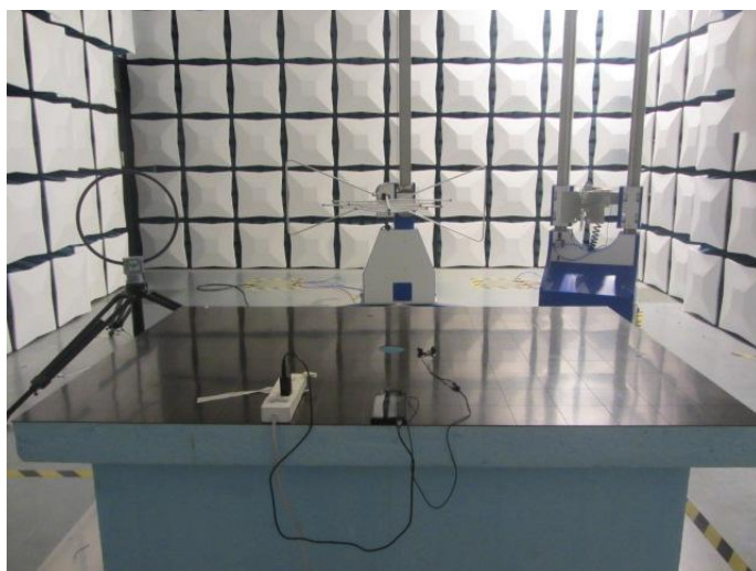
Radiated Spurious Emission (30M~1GGHz)
