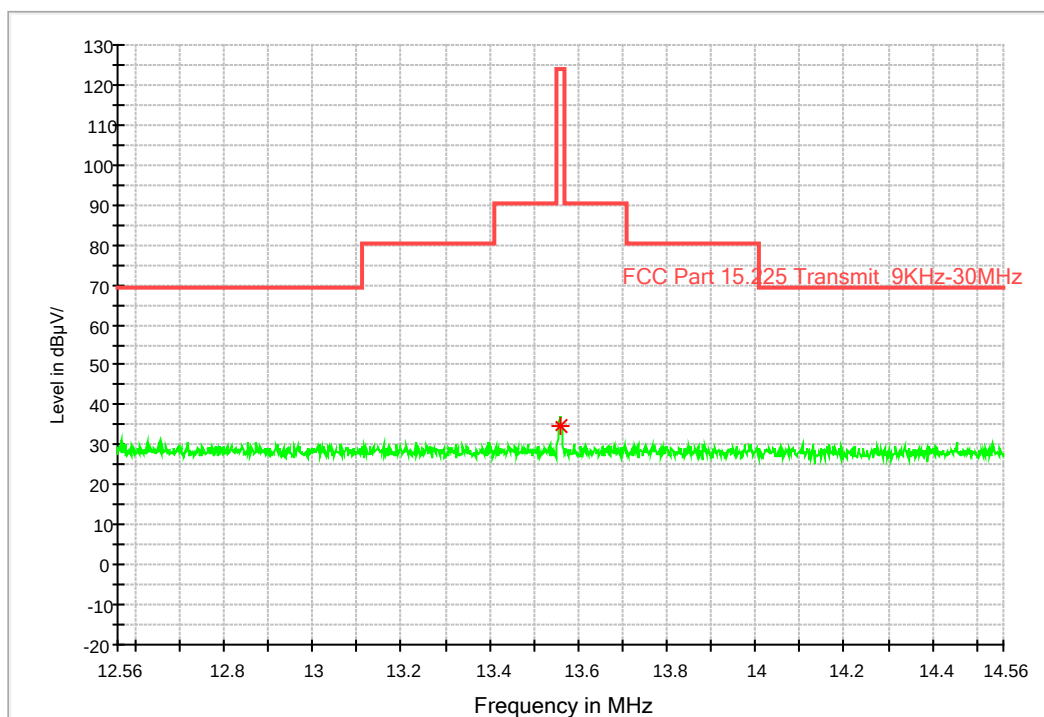
FCC Loop Antenna 9KHz-30MHz
