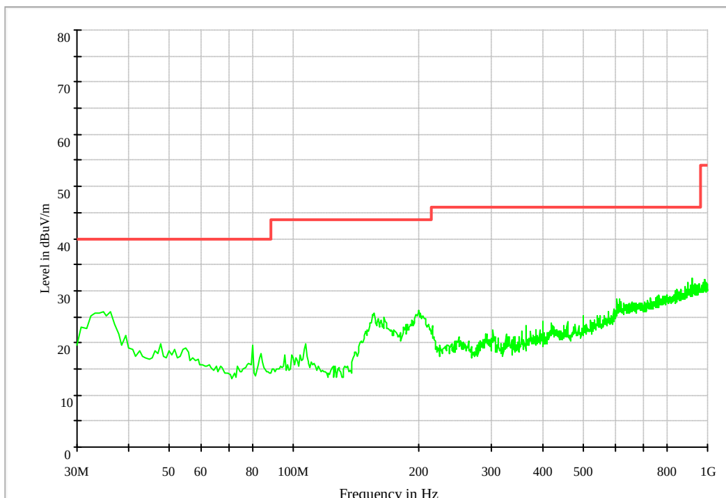
FCC CLASS B RE 30MHz-1GHz
