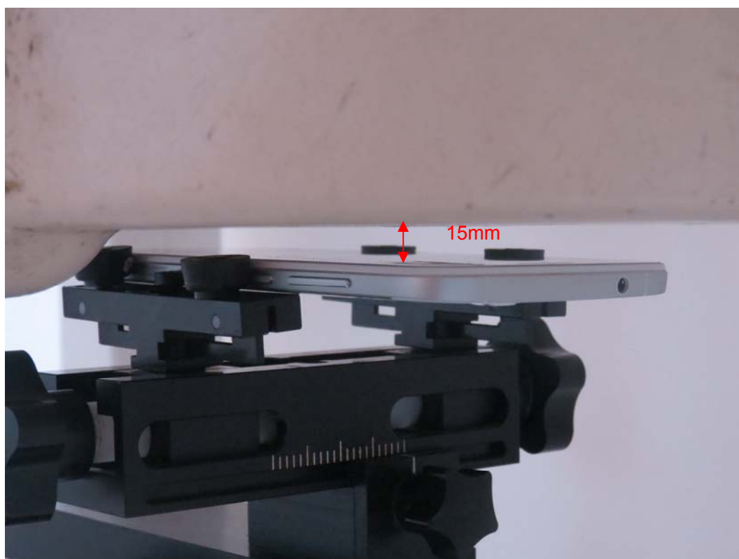
Picture 17: Front Side, the distance from handset to the bottom of the Phantom is 15mm
