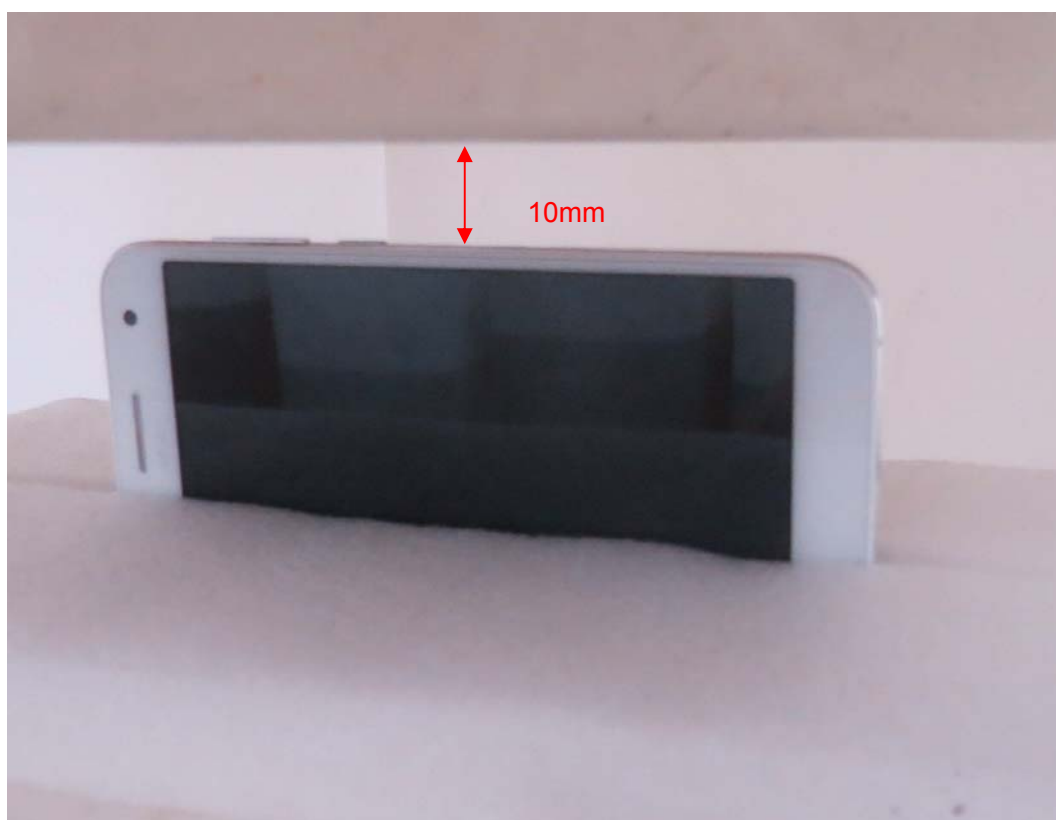
Picture 20: Right Edge, the distance from handset to the bottom of the Phantom is 10mm
