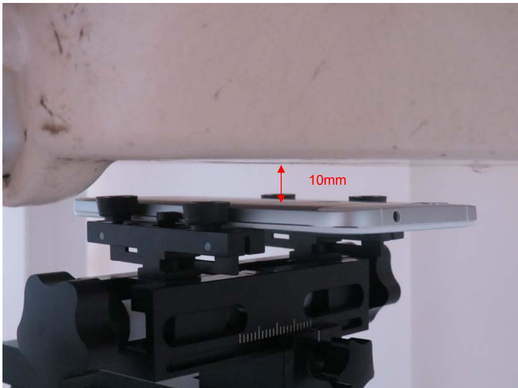
Picture 16: Back Side, the distance from handset to the bottom of the Phantom is 10mm
