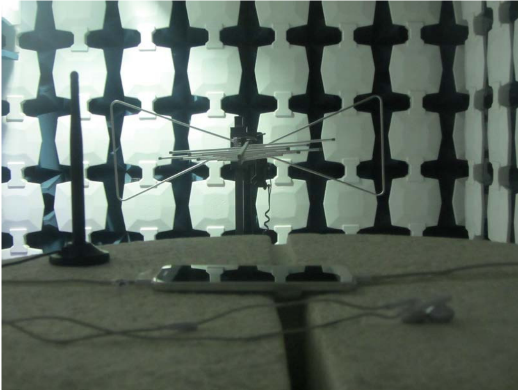
Radiated Spurious Emission (below 3GHz)
