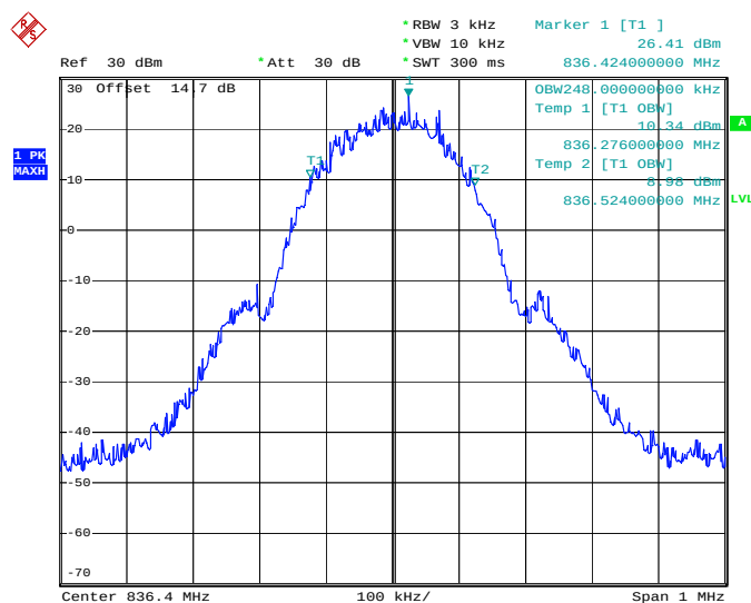
99% Occupied Bandwidth Plot on Channel 189
