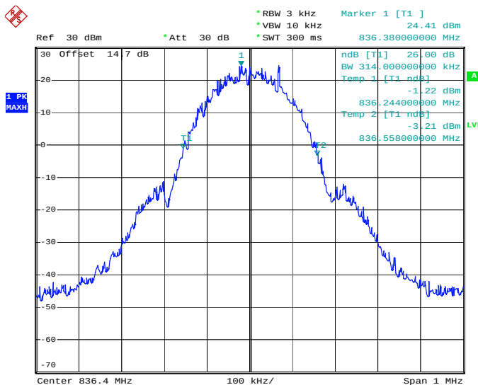
26dB Bandwidth Plot on Channel 189
