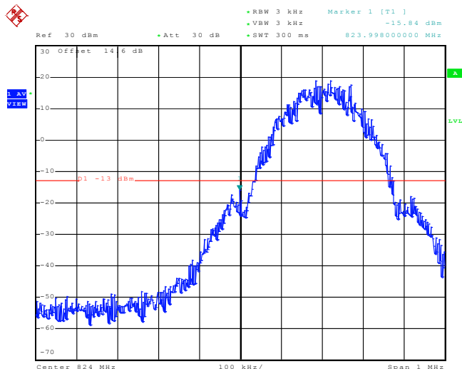
Lower Band Edge Plot on Channel 128
