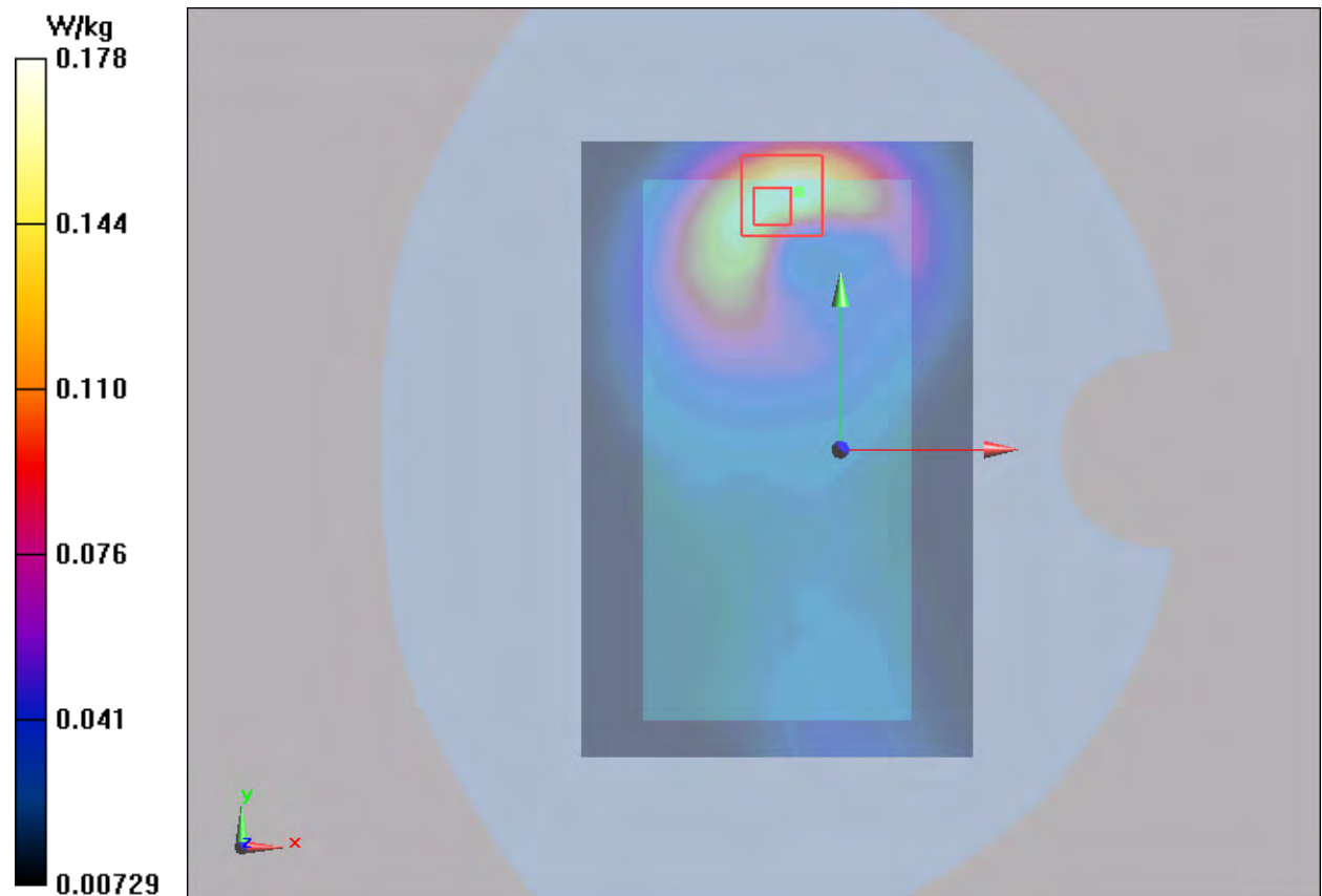
Figure 59 Body, Back Side, LTE Band 17 50%RB Channel 23790
