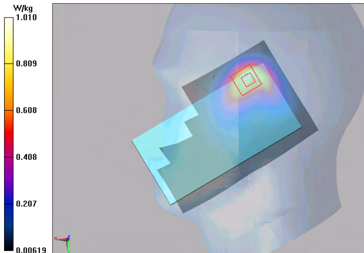
Figure 45 Right Hand Touch Cheek LTE Band 4 1RB Channel 20300
