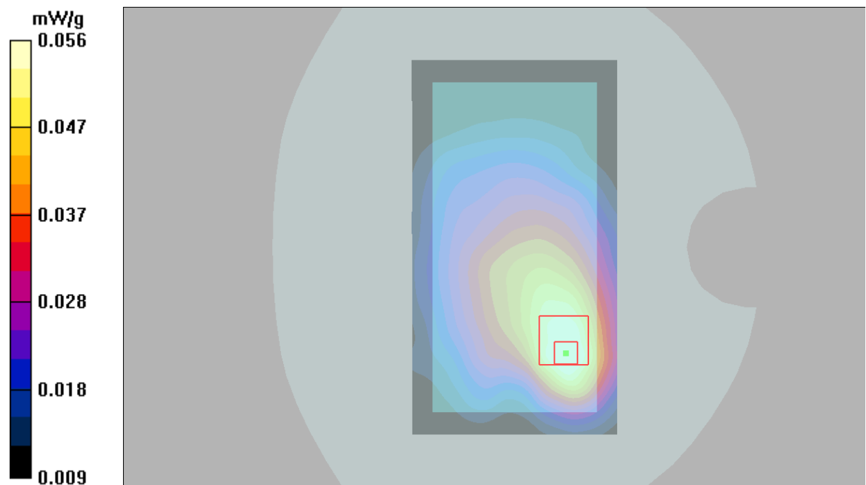
Figure 97 Body, Back Side, LTE Band 17 1RB Channel 23790
