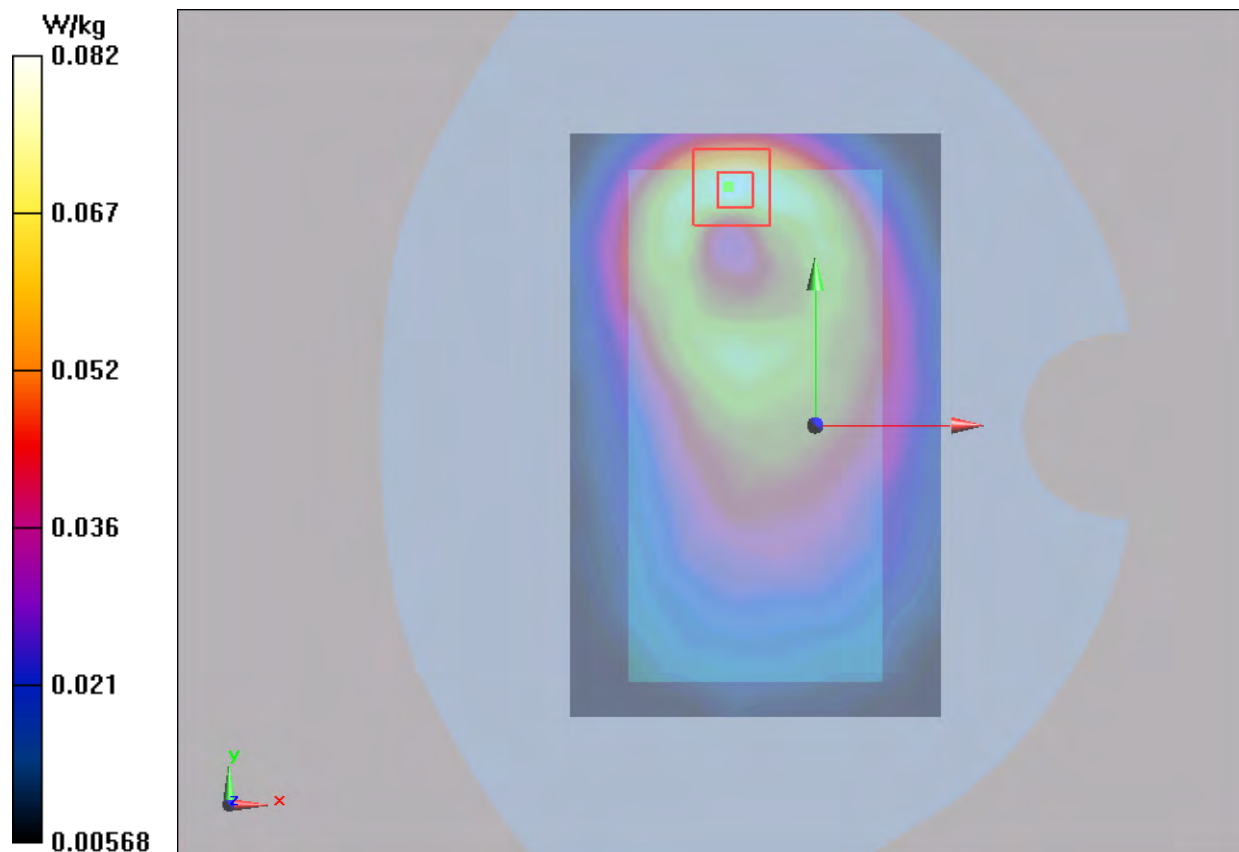
Figure 58 Body, Front Side, LTE Band 17 50%RB Channel 23790
