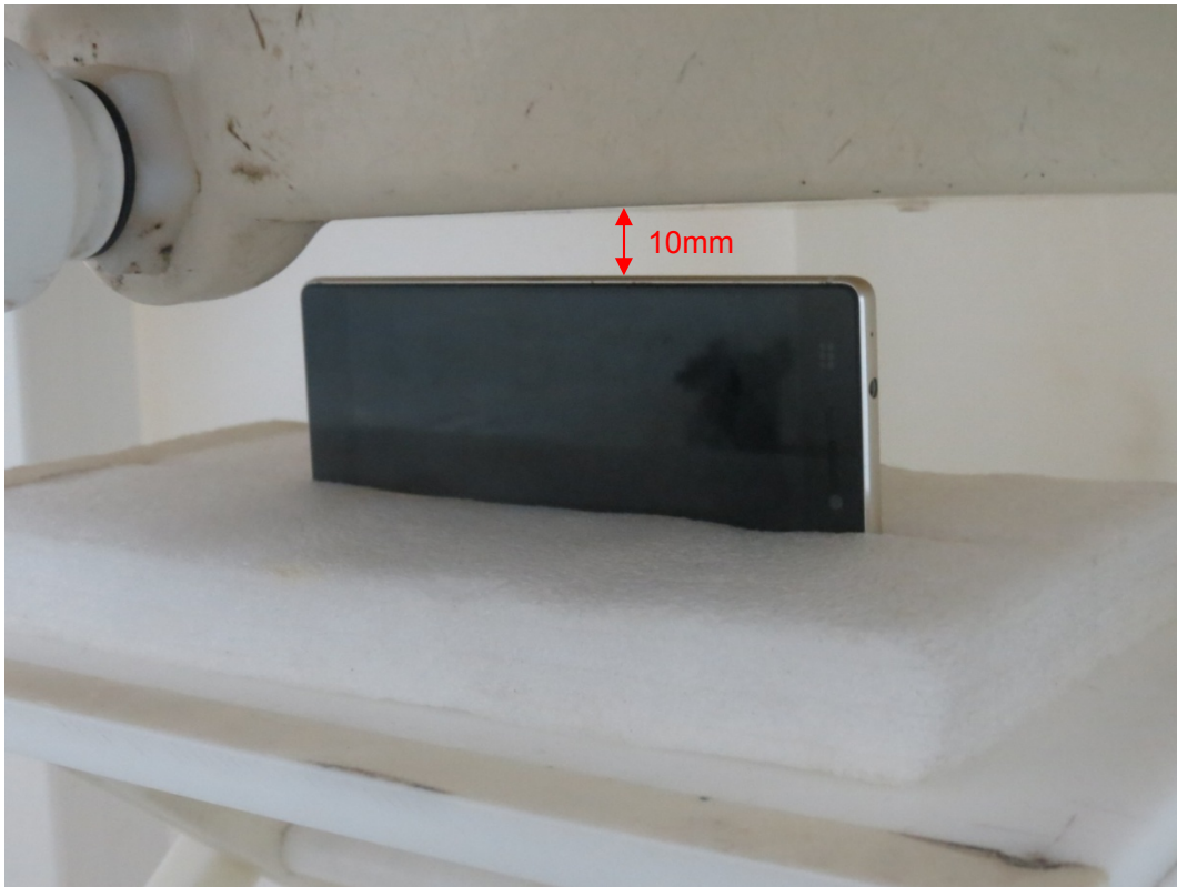
Picture 22: Left Side, the distance from handset to the bottom of the Phantom is 10mm
