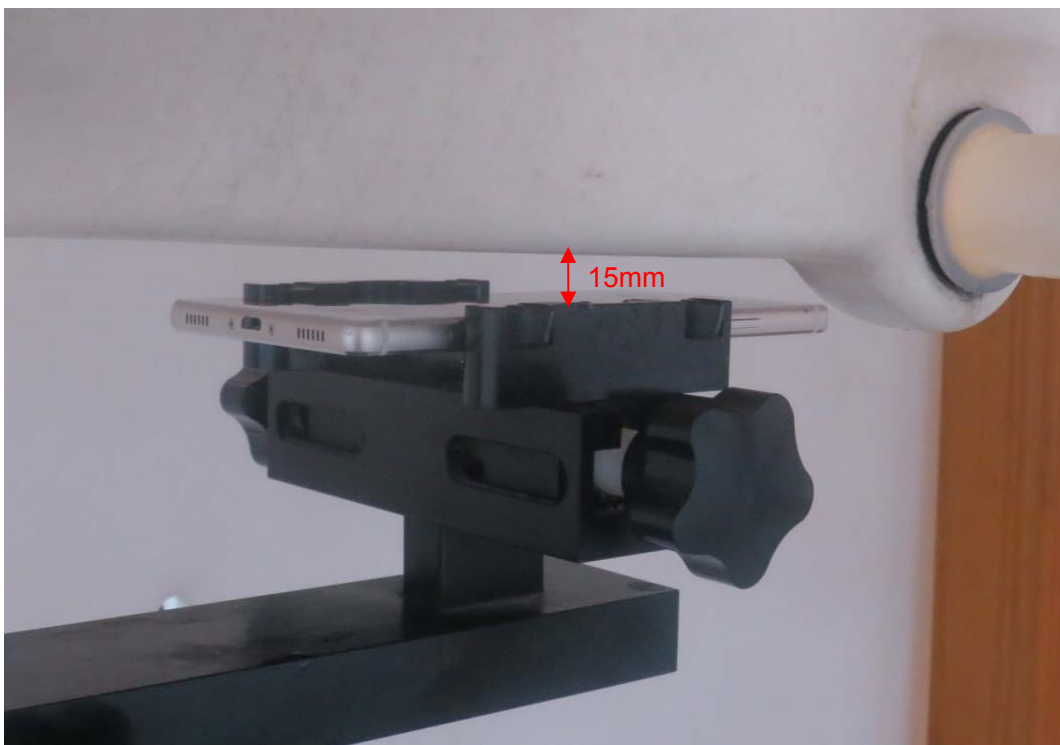
Picture 19: Front Side, the distance from handset to the bottom of the Phantom is 15mm
