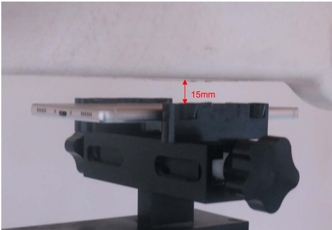
Picture 18: Back Side, the distance from handset to the bottom of the Phantom is 15mm
