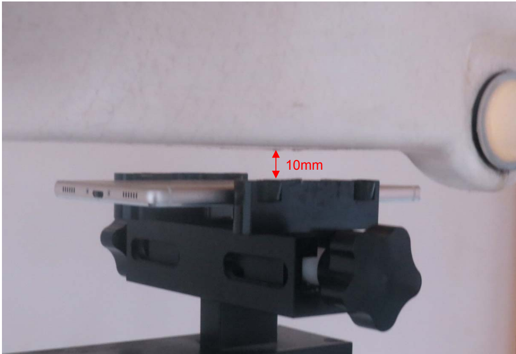
Picture 20: Back Side, the distance from handset to the bottom of the Phantom is 10mm
