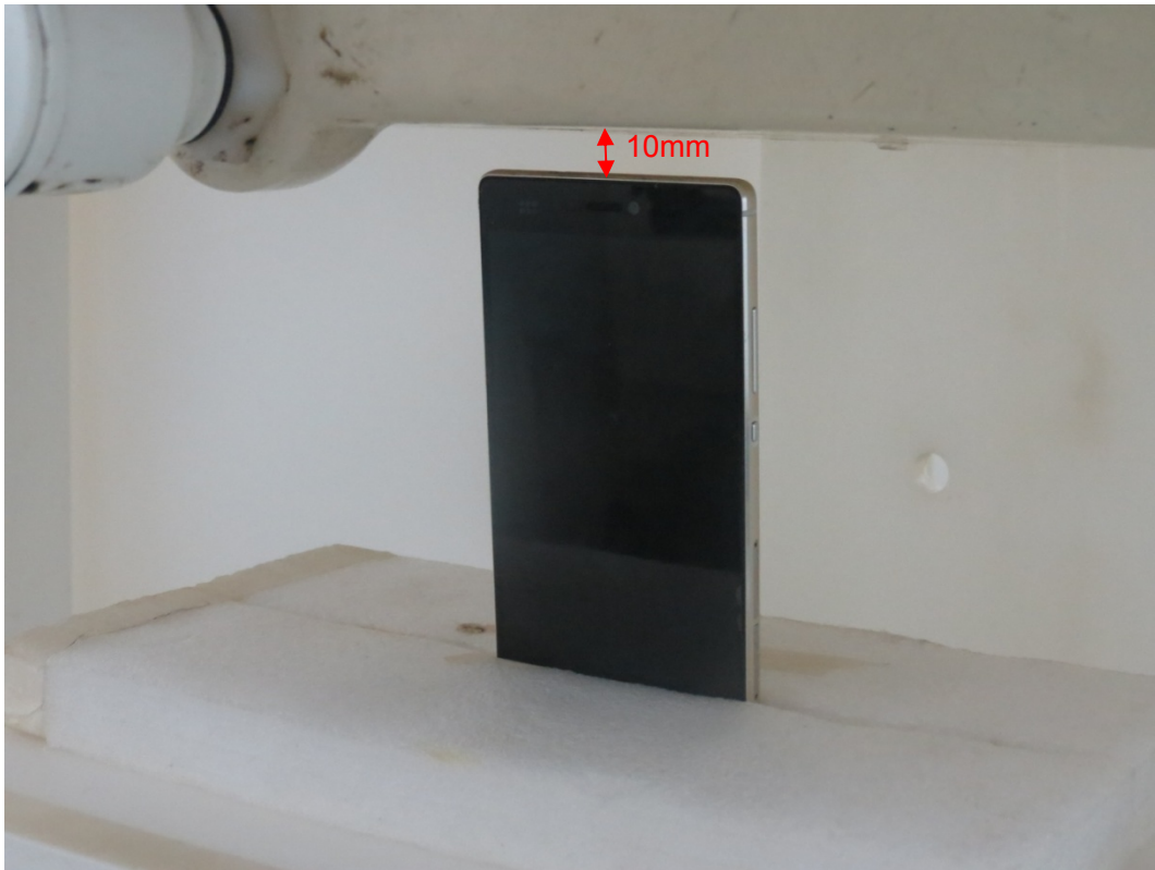
Picture 24: Top Side, the distance from handset to the bottom of the Phantom is 10mm
