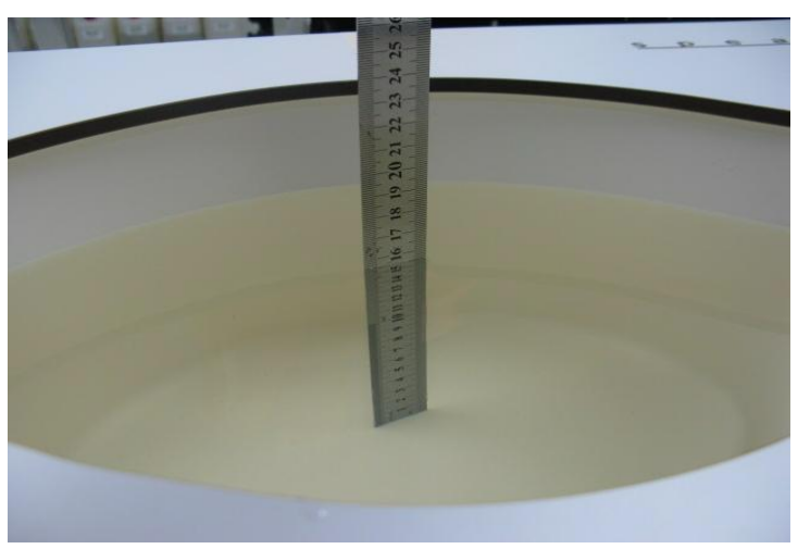
Photo 21: MSL 1900MHz depth (15.2cm)
