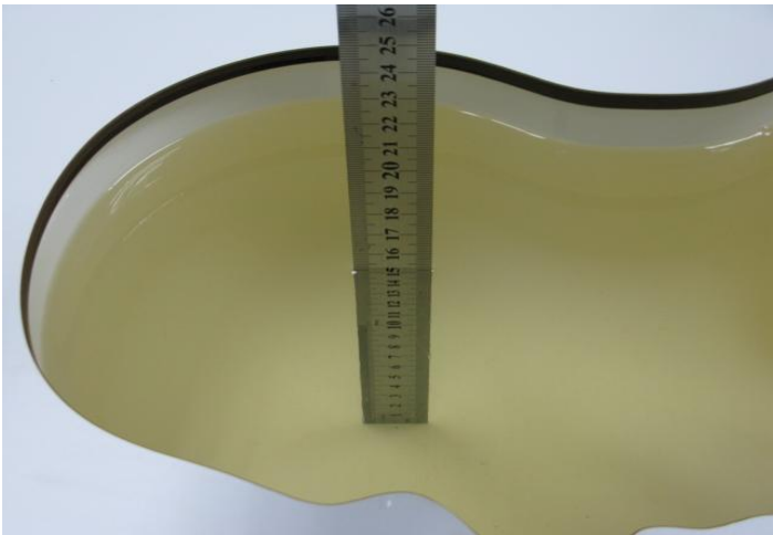
Photo 24: HSL 2600MHz depth (15.1cm)
