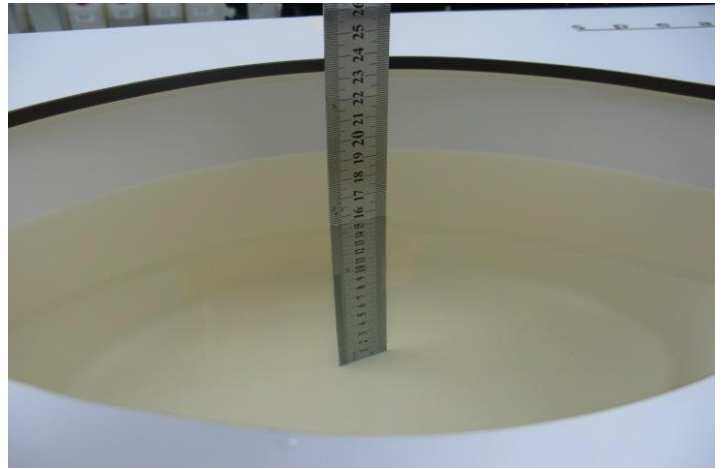
Photo 19: MSL 1750MHz depth (15.2cm)
