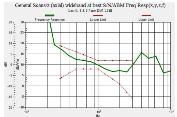
CDMA BC1/600CH-Main Antenna
