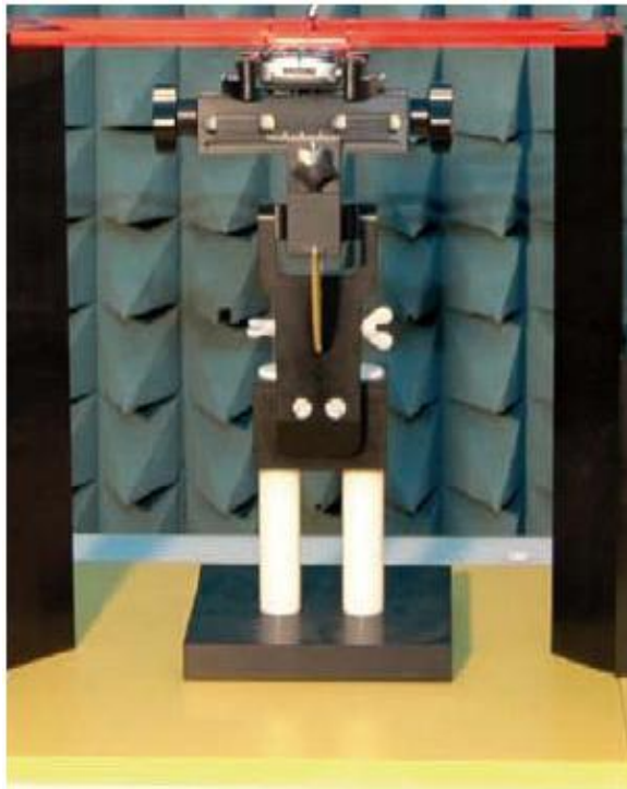
Fig. 4 HAC Phantom &amp; Device Holder
