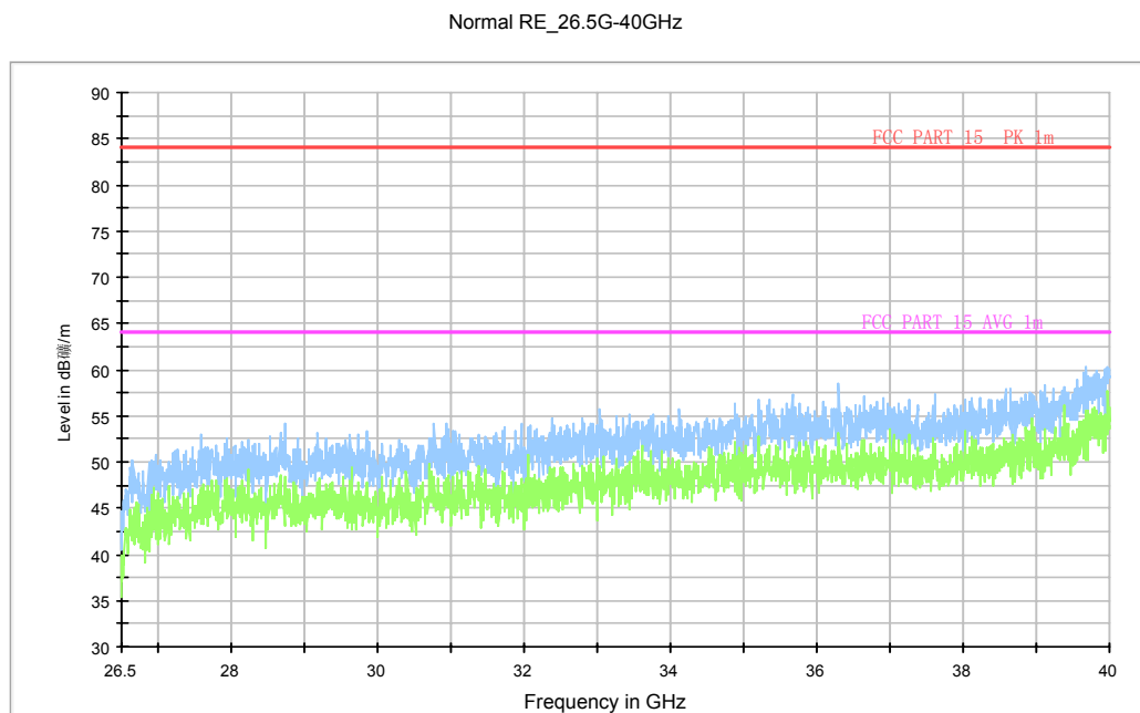
Fig. 74 Radiated Spurious Emission (802.11a, ch56, 26.5 GHz-40 GHz)
