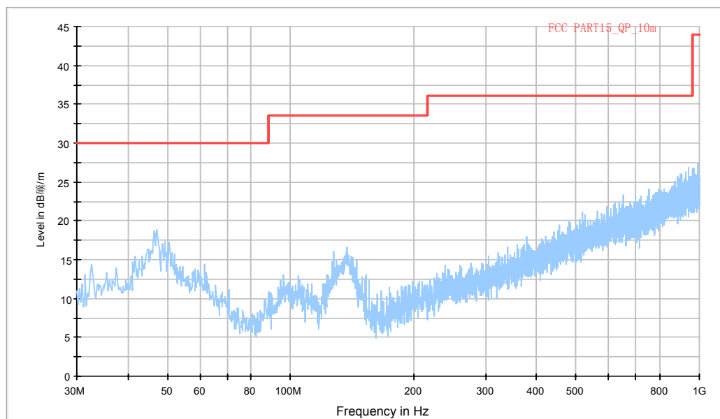
Normal RE_30M-1GHz_10m
