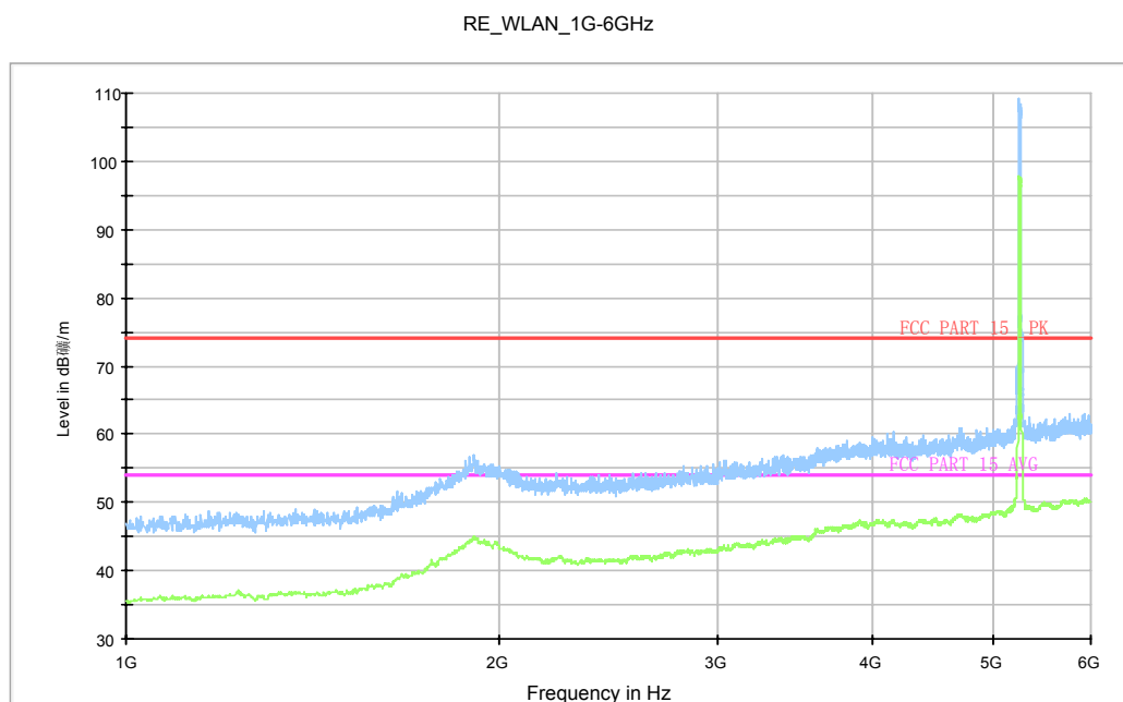
Fig. 77 Radiated Spurious Emission (802.11n-HT20, ch52, 1 GHz-6 GHz)
