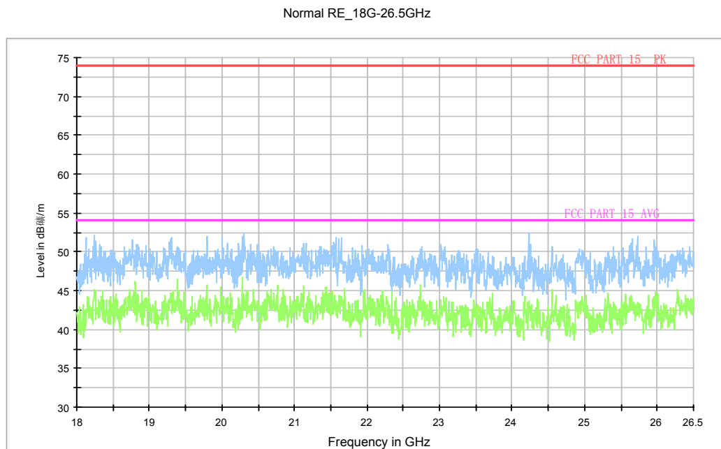
Fig. 132 Radiated Spurious Emission (802.11n-HT40, ch118, 18 GHz-26.5 GHz)
