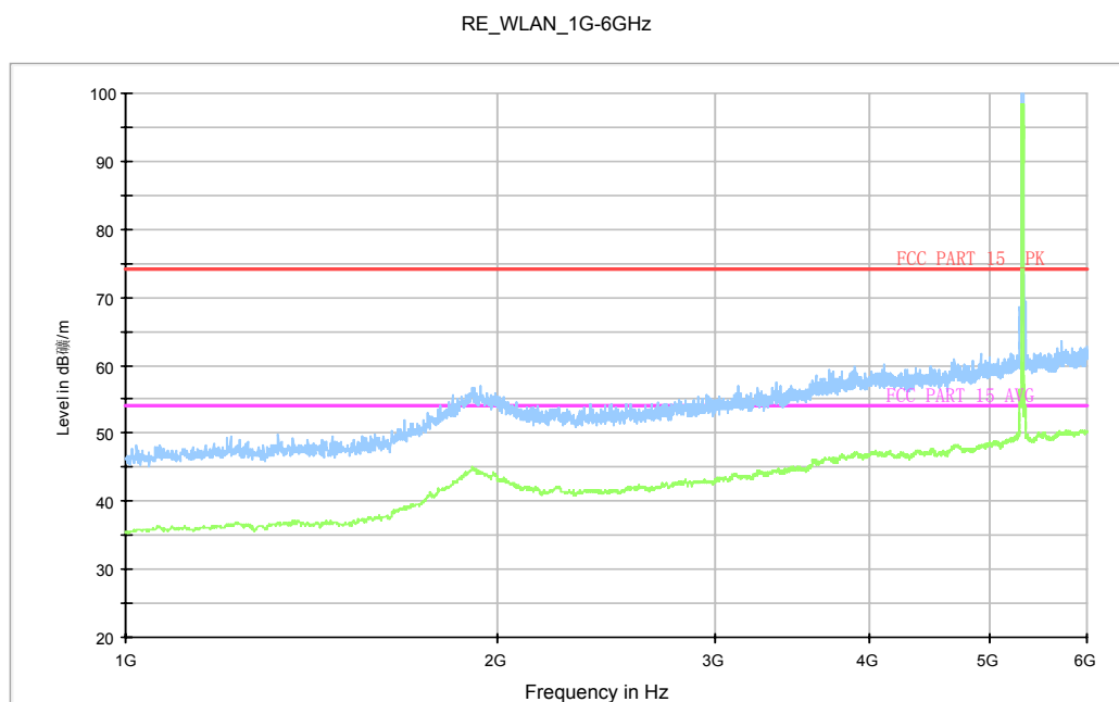
Fig. 75 Radiated Spurious Emission (802.11a, ch64, 1 GHz-6 GHz)
