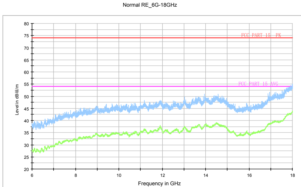
Fig. 131 Radiated Spurious Emission (802.11n-HT40, ch118, 6 GHz-18 GHz)
