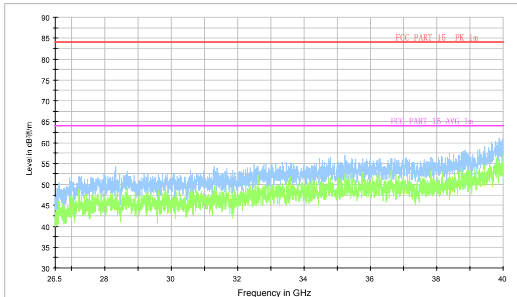
Normal RE_26.5G-40GHz
