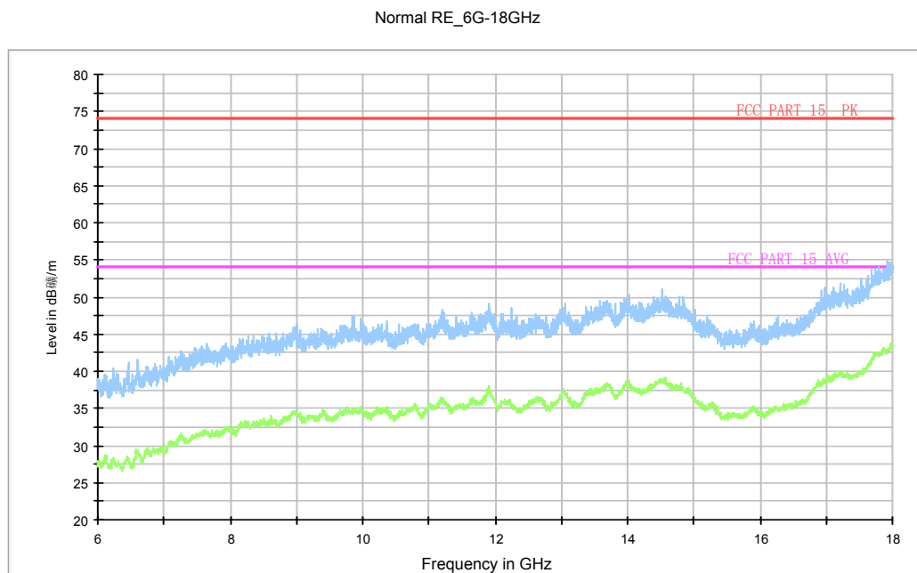
Fig. 76 Radiated Spurious Emission (802.11a, ch64, 6 GHz-18GHz)
