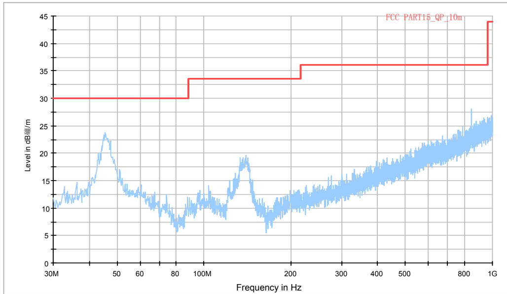
Normal RE_30M-1GHz_10m
