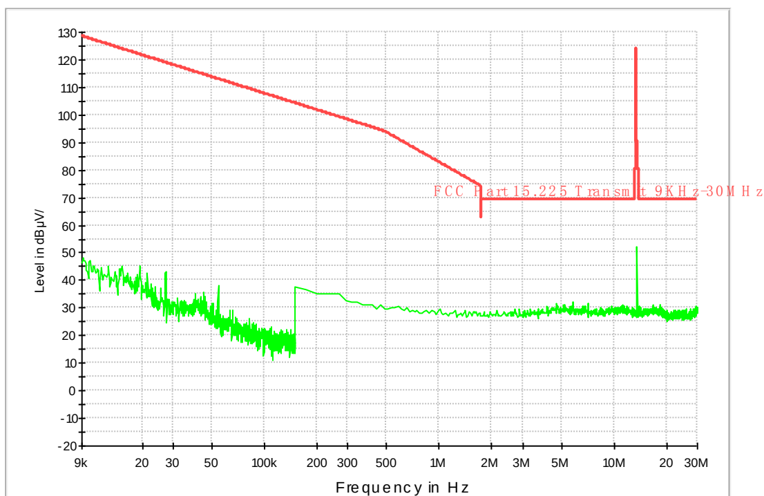
FCC Loop Antenna 9KHz-30MHz
