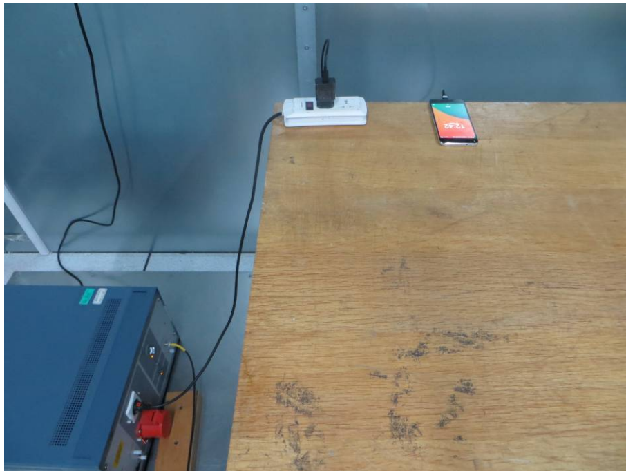
10. Conducted Emission (Part 15B Charging mode)
