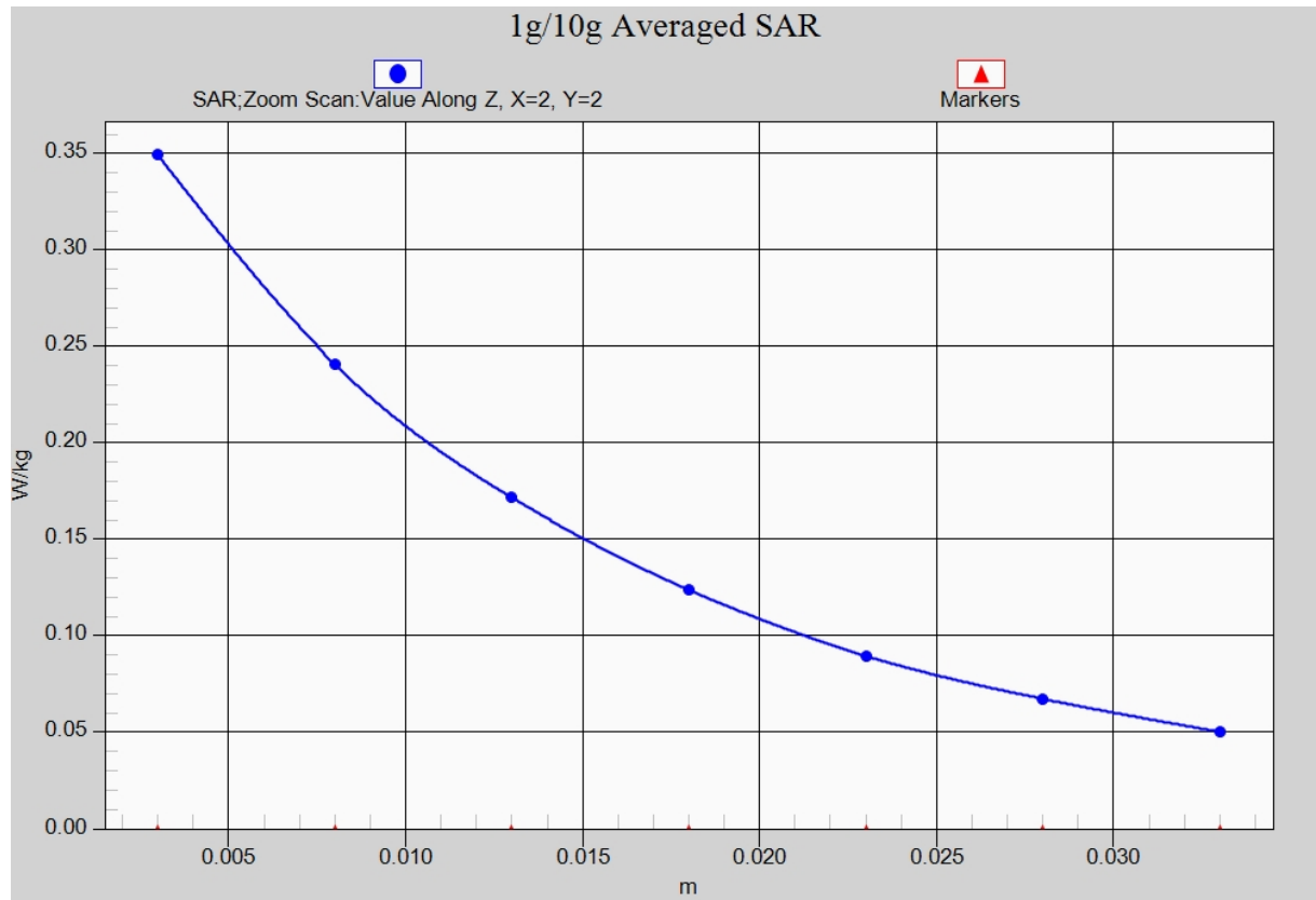
Fig. 19-1 Z-Scan at power reference point (LTE Band4)
