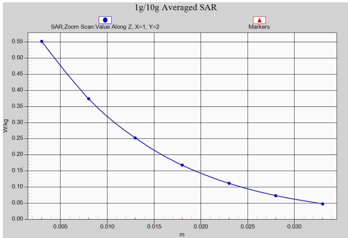
Fig. 15-1 Z-Scan at power reference point (WCDMA1900)
