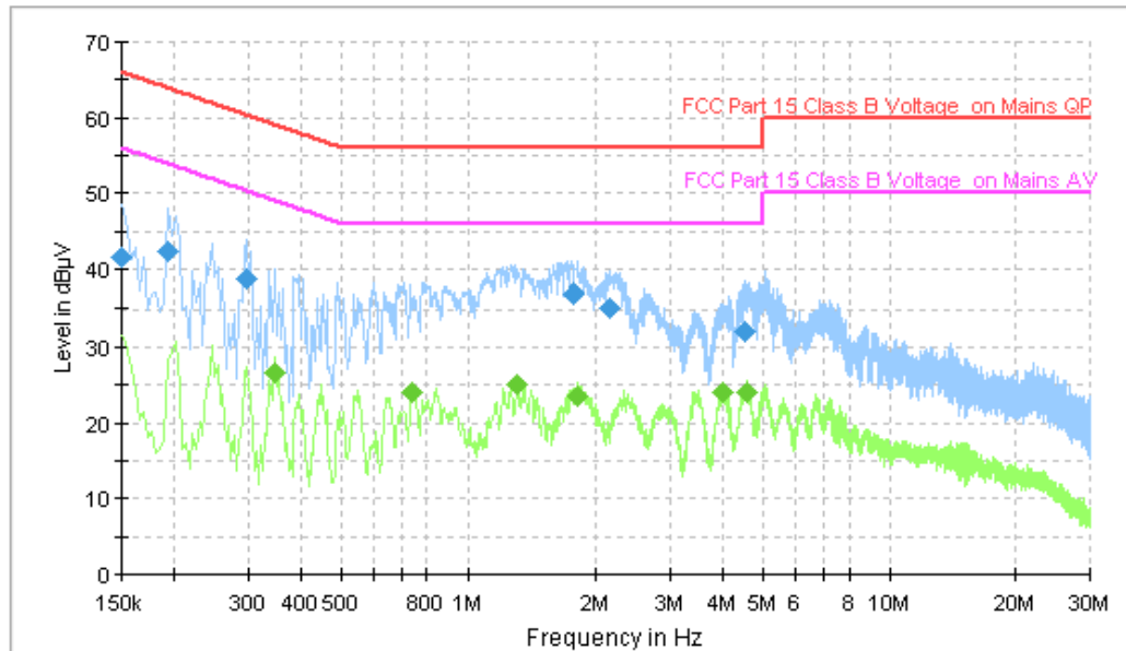
Figure A.37 Conducted Emission
