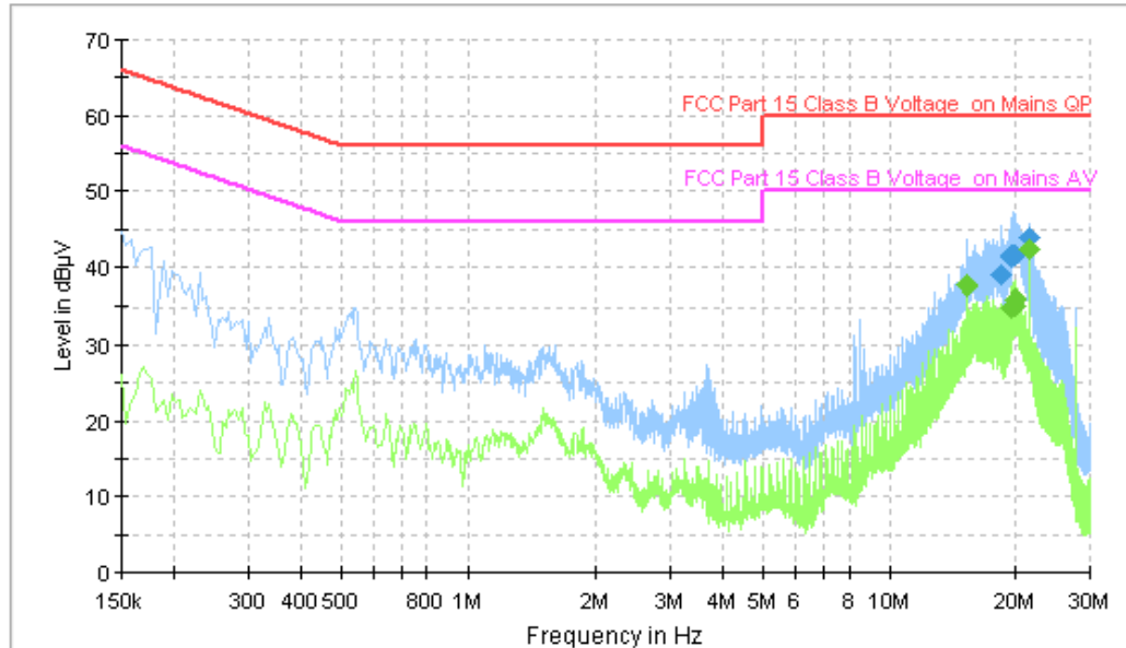
Figure A.35 Conducted Emission
