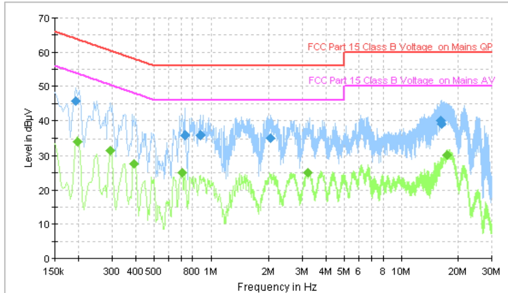
Figure A.42 Conducted Emission
