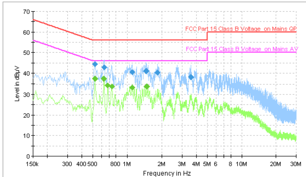
Figure A.40 Conducted Emission
