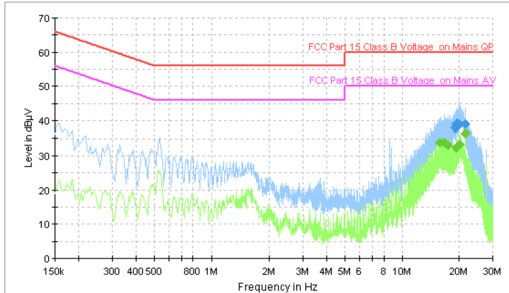
Figure A.33 Conducted Emission
