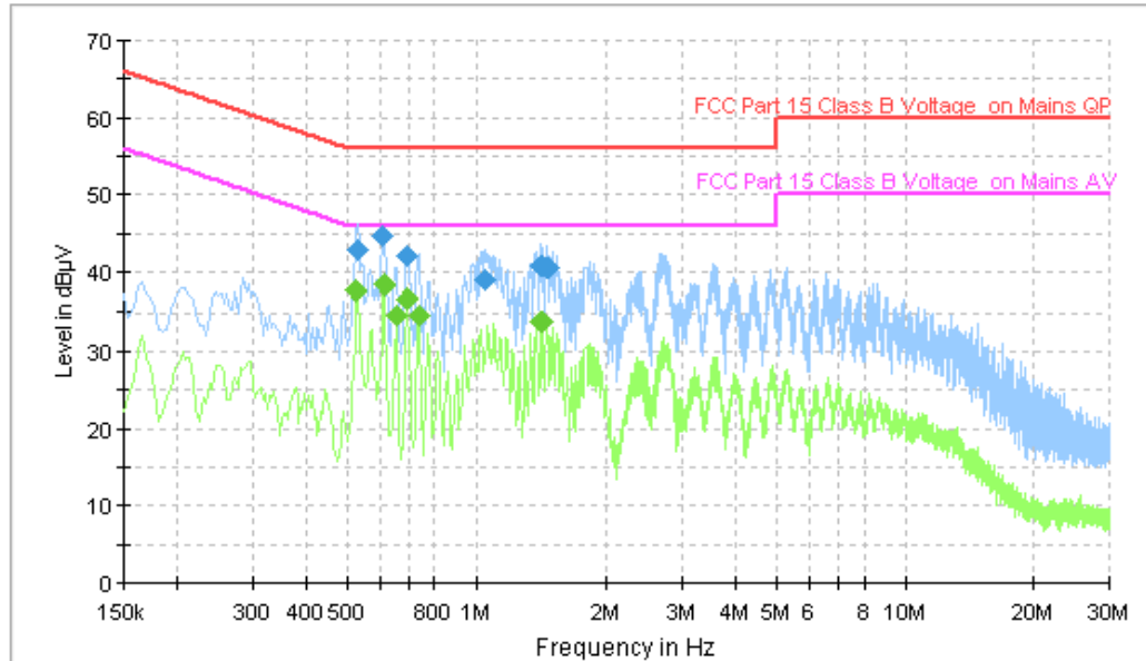
Figure A.36 Conducted Emission
