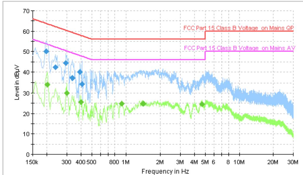
Figure A.41 Conducted Emission
