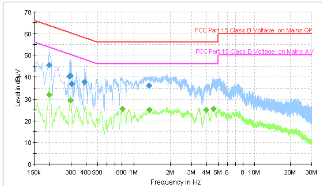
Figure A.30 Conducted Emission
