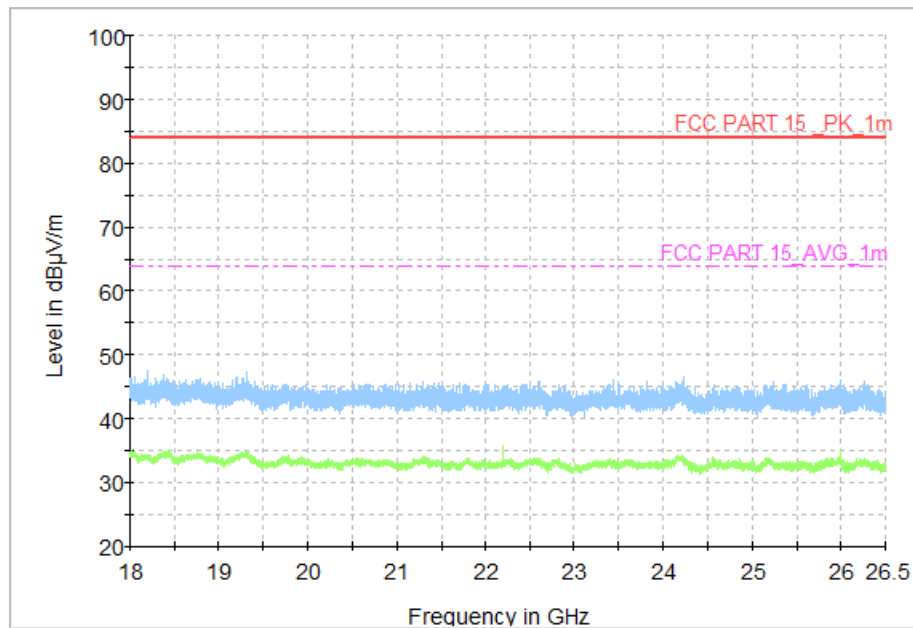
Figure A.23 Radiated Emission from 18GHz to 26.5GHz
