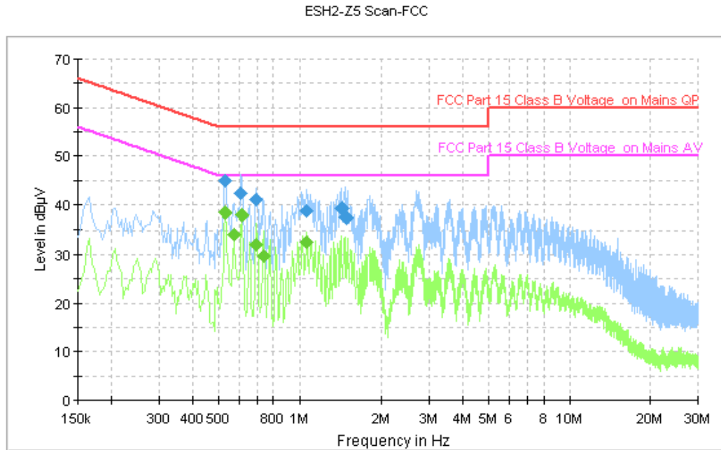
Figure A.39 Conducted Emission
