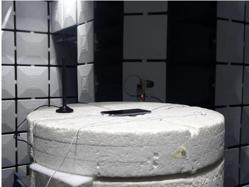
Radiated Spurious Emission (18GHz to26.5GHz)
