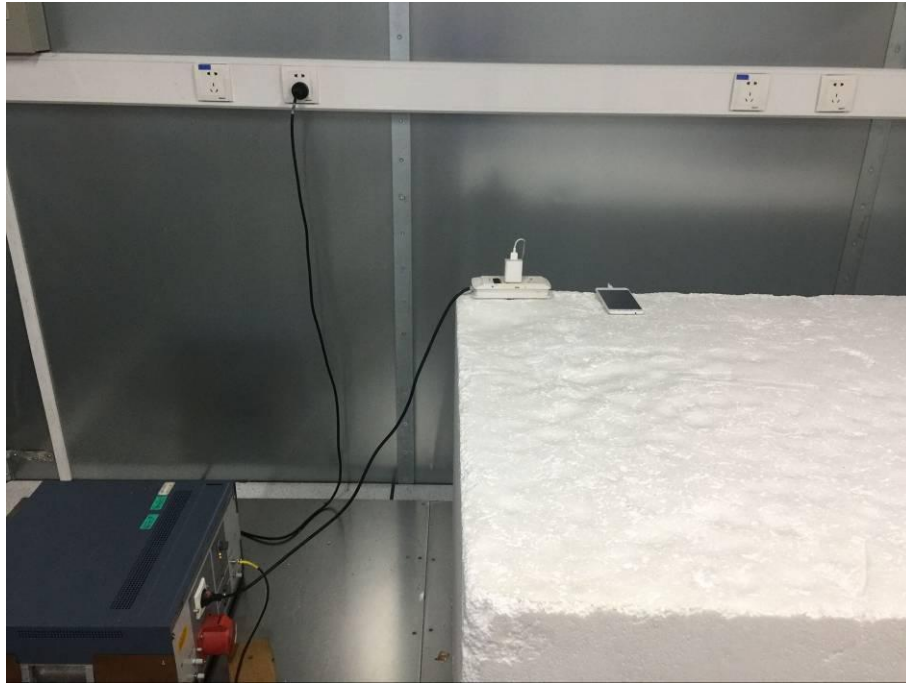
11. Conducted Emission (Part 15B Charging mode)
