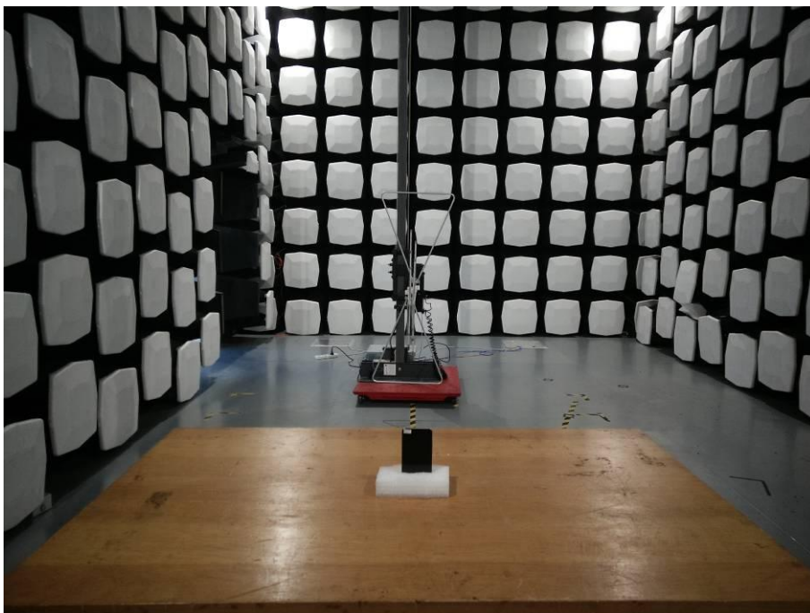
6. Radiated Emissions (Part 15E) (30M-1GHz)
