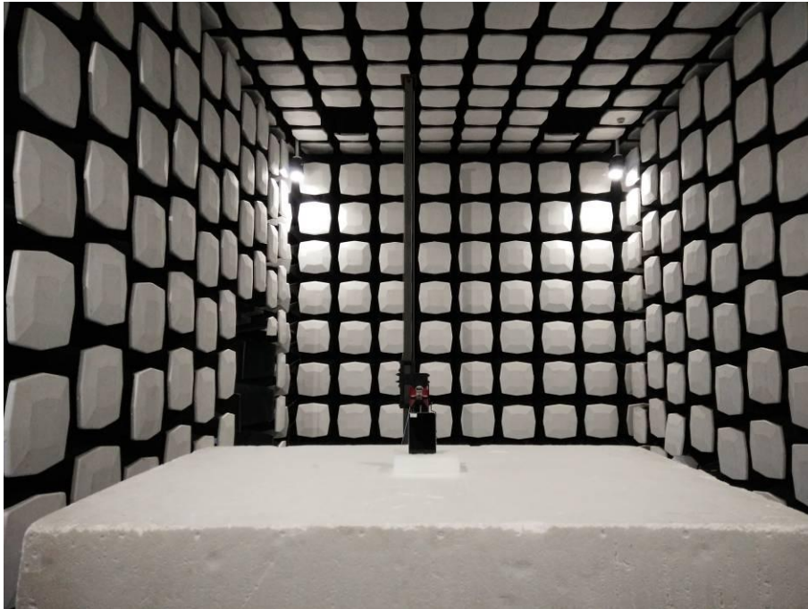
7. Radiated Emissions (Part 15E) (1-18GHz)
