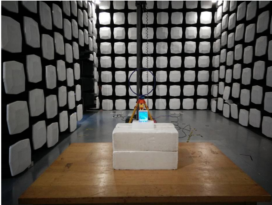
5. Radiated Emissions (Part 15E) (9kHz-30MHz)
