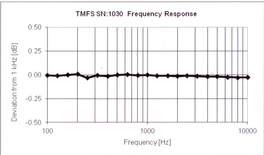
Fig. 2 Frequency response 100 to 10'000 Hz
