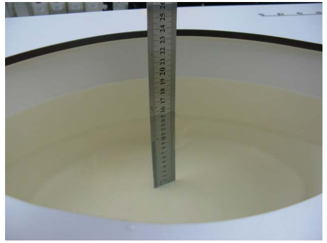
Photo 14: MSL1900MHz depth (15.1cm)
