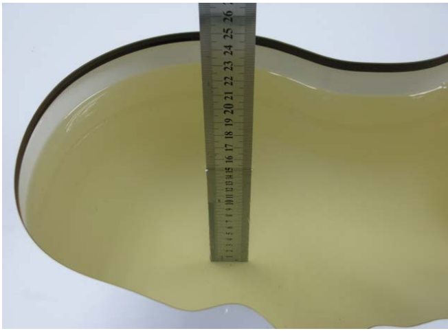
Photo 13: HSL1900MHz depth (15.2cm)
