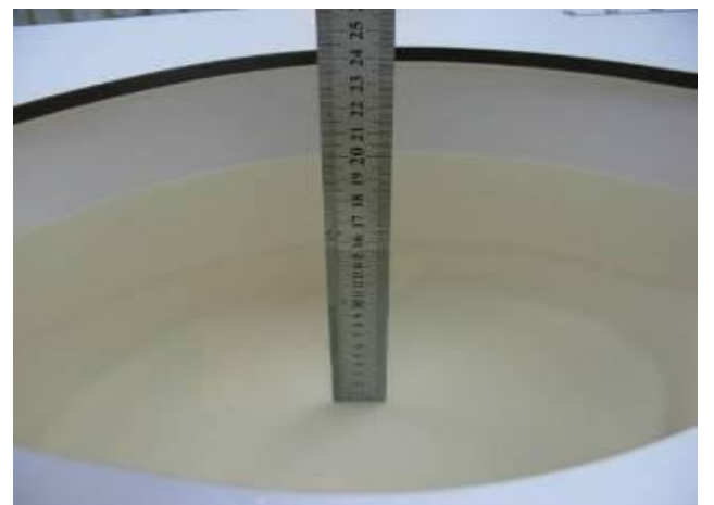
Photo 16:MSL 2450MHz depth (15.1cm)
