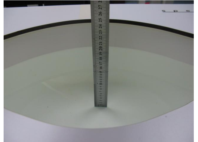
Photo 13:MSL 1900MHz depth (15.1cm)
