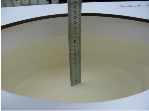
Photo 12: MSL 1750MHz depth (15.2cm)
