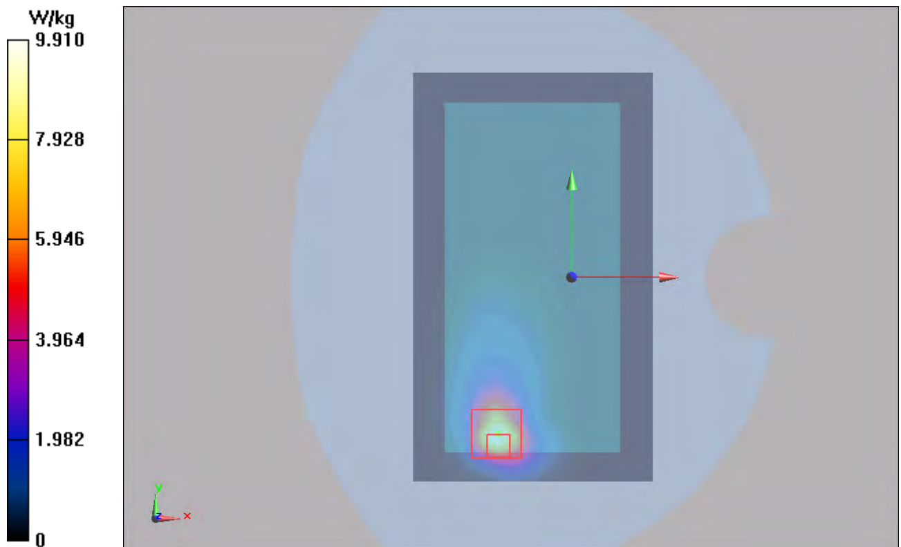
Figure 53 Body, CDMA BC1 EVDO Back Side Channel 600
