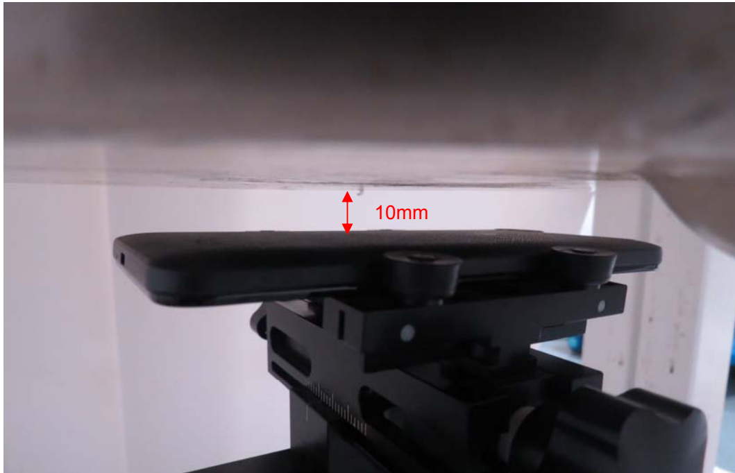
Picture 17: Back Side, the distance from handset to the bottom of the Phantom is 10mm
