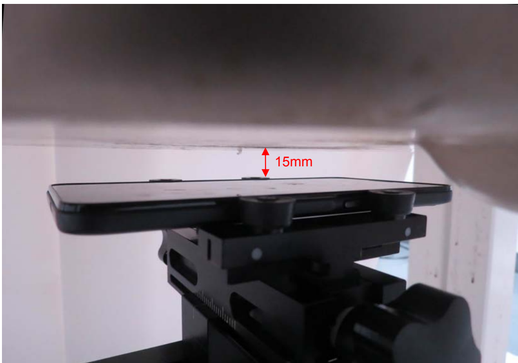
Picture 16: Front Side, the distance from handset to the bottom of the Phantom is 15mm
