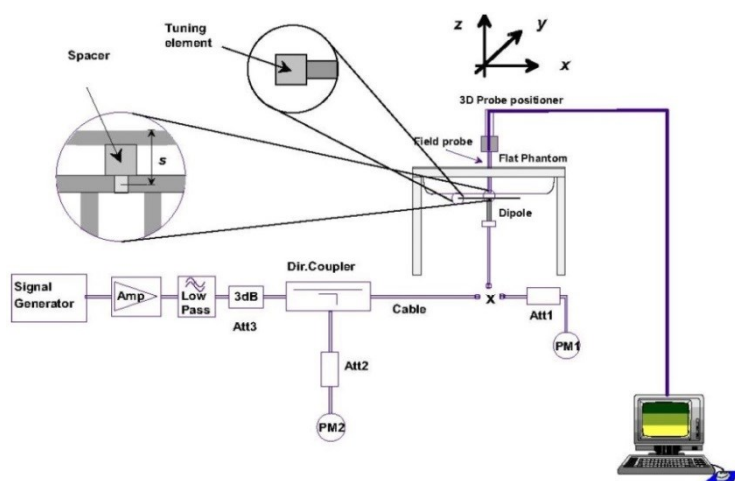
Fig 11.3.1 System Performance Check Setup
