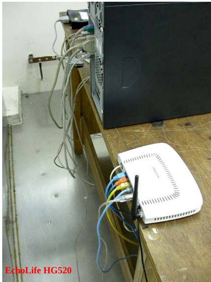
Photo 2: Conducted Emission Test set-up photo
