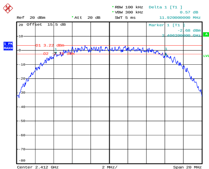
Mode 1 : 6 dB Bandwidth Plot on 802.11b Channel 01- Chain B
